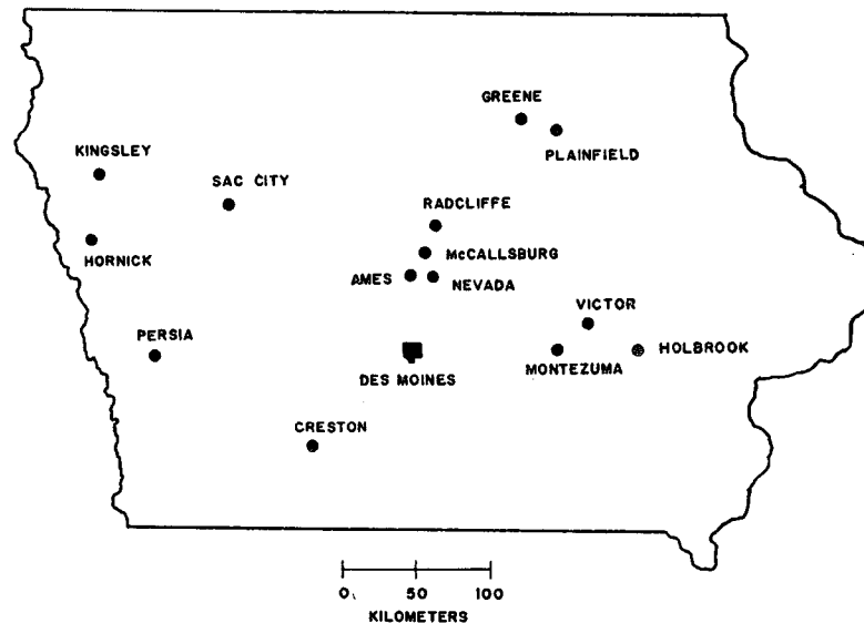
FIG. 1. Map of Iowa showing relative locations of severe weather events studied in this investigation.
