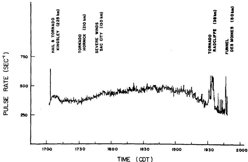
Fig. 7. Electromagnetic pulse rate vs time for Storm No. 5 of 14 July 1970. The pulse rates were obtained by averaging over 20 sec.
