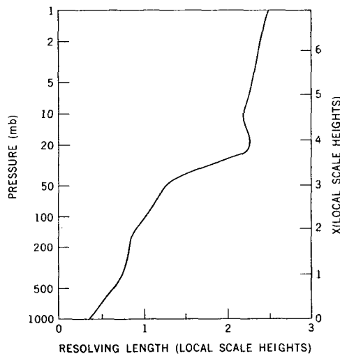
FIG. 6. The resolving length plotted as a function of atmospheric level. The resolving length provides a measure of vertical resolution.
