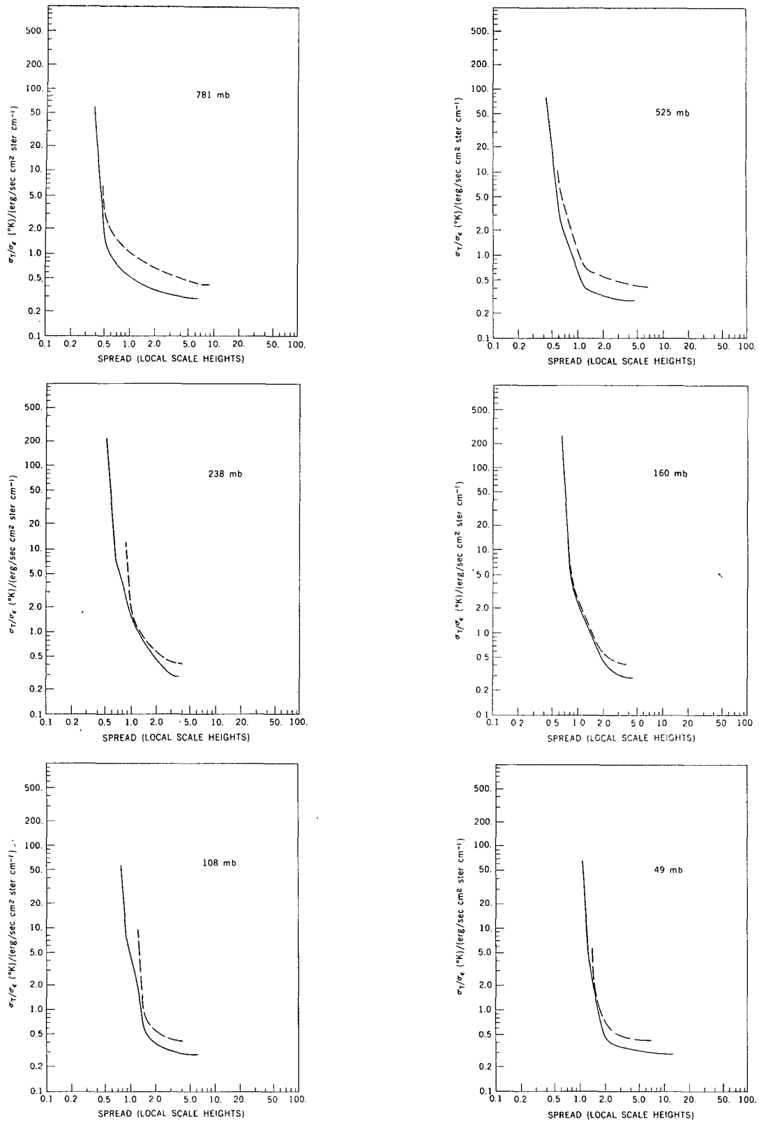
FIG. 2. Tradeoff curves for the 667 cm -1 CO 2 absorption band. \sigma_T is the standard deviation of the temperature error due to a random measurement error with standard deviation \sigma_e . The atmospheric pressure level to which each curve pertains is indicated. The solid curves are for a set of 16 spectral intervals while the broken curves are for a 7-interval set.
