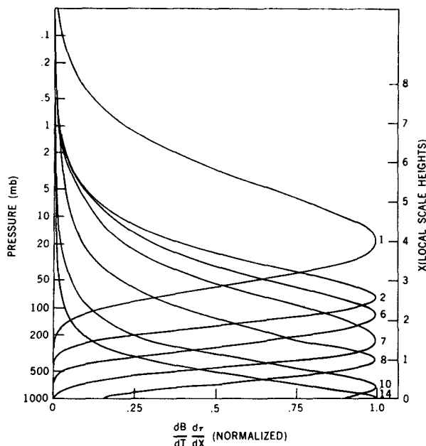
FIG. 1. Radiative transfer kernels for the 667 \text{cm}^{-1} \text{CO}_2 absorption band. The numbers labeling the curves refer to spectral intervals listed in Table 1.
