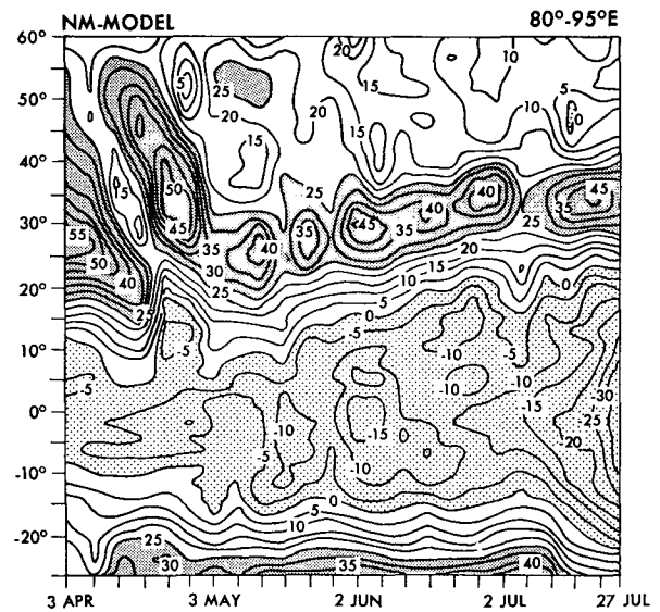
FIG. 5.3. Latitude-time section of zonally averaged (80–95°E) 5-day mean zonal winds ( \text{m s}^{-1} ) at the 190 mb level of the NM-model.
