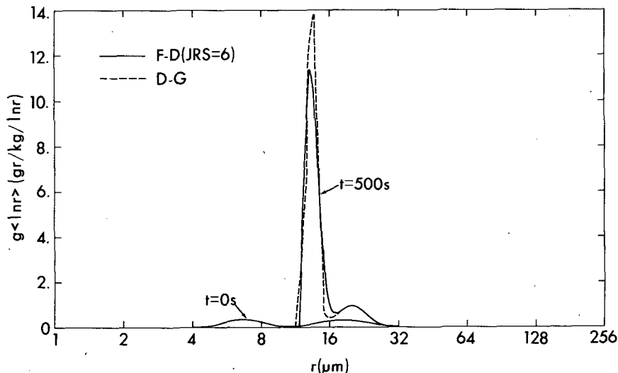
FIG. 10. As in Fig. 2 except for case 4.
