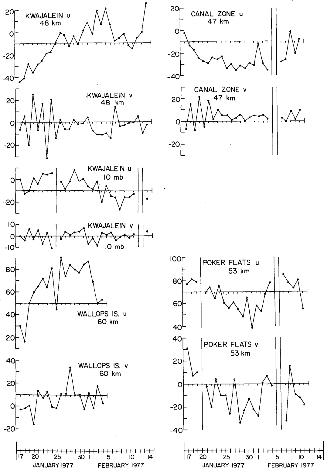
FIG. 2. Time series of u (zonal) and v (meridional) wind at selected stations and levels as shown. All winds are in m\ s^{-1} . Vertical lines denote missing data. The lines connecting data points are to aid in viewing the data as a time series and are not intended as interpolations. The approximate time of day (GMT) for the rocket launch was 2300 for Kwajalein ( 9^{\circ}N , 168^{\circ}E ), 1700 for the Canal Zone ( 9^{\circ}N , 80^{\circ}W ), 1600 for Wallops Island ( 38^{\circ}N , 76^{\circ}W ) and 2200 for Poker Flats ( 65^{\circ}N , 148^{\circ}W ).
