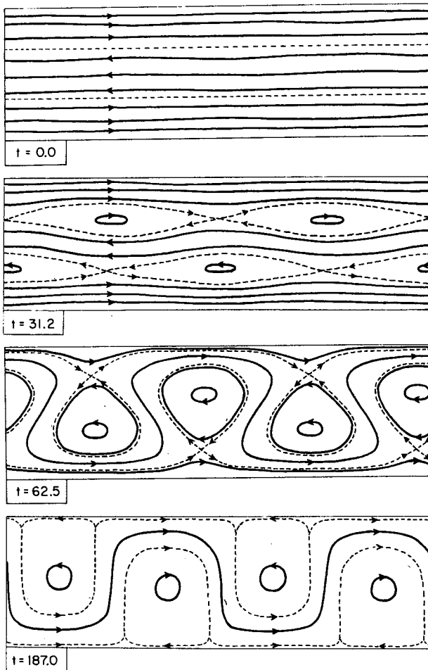
FIG. 2. Instability of \bar{u} = \cos y , with y_1 = 0, y_2 = 2\pi for k^2 = 0 . In Figs. 2-7 the x axis is compressed, such that a unit length appears \frac{1}{6} as long in the horizontal direction as in the vertical direction. Solutions are obtained on a 64 \times 64 grid. The dashed lines represent the critical streamlines; the shapes near the cusps are uncertain.
