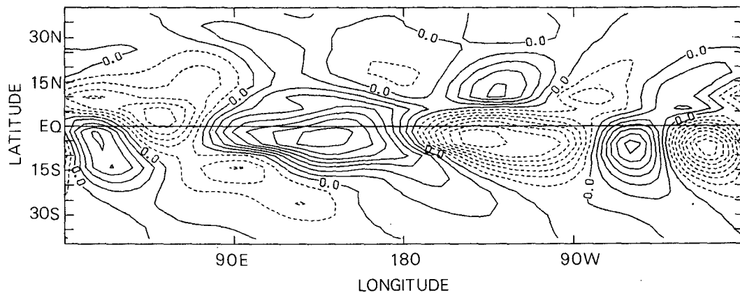
FIG. 7. Contours of the synthetic horizontal heating distribution of heating based upon climatological December–February values of the outgoing flux at the top of the atmosphere. See text for explanation. The quantity contoured here is the heating rate ( K \text{ day}^{-1} ) for the MC profile at the level of maximum heating. The contour interval is 0.5 K \text{ day}^{-1} and negative contours are dashed.
