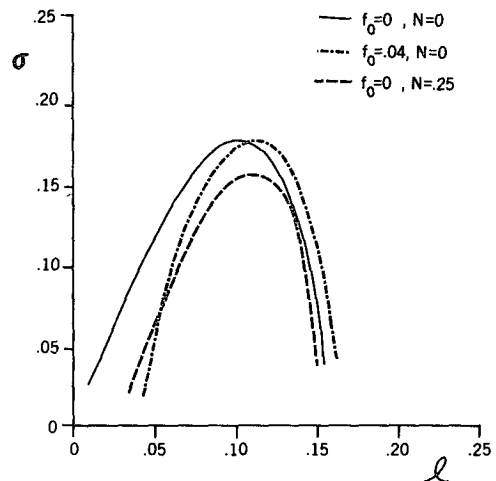
FIG. 14. Nondimensional growth rate \sigma(I_m\omega) of the shear-gravity mode as a function of nondimensional horizontal wavenumber for the case \xi_0/N_s = 0.5 and H/2a = 1 . The curves are labeled with values of the nondimensional Coriolis parameter and the nondimensional outer region Brunt-Väisälä frequency. See text for normalizations.
