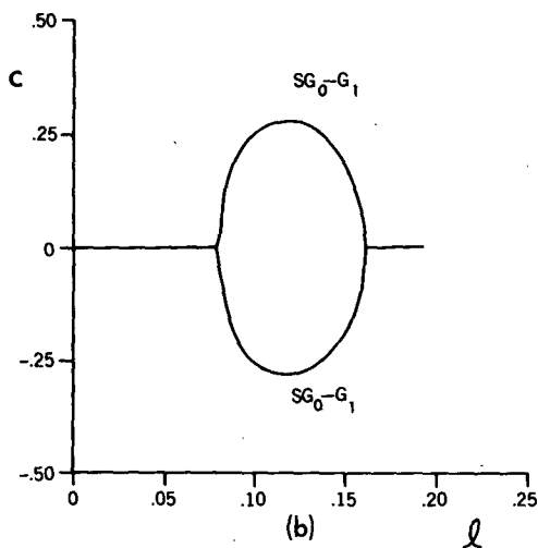
FIG. 11. (a) Nondimensional growth rate \sigma(l_m\omega) and (b) phase speed c(R\phi\omega/l) of the shear-gravity mode SG_0 and the first two modified gravity modes, G_1 and G_2 , as a function of normalized horizontal wavenumber l for the case \xi_0/N_s = 0.8 and H/2a = 1 . See text for normalizations.
