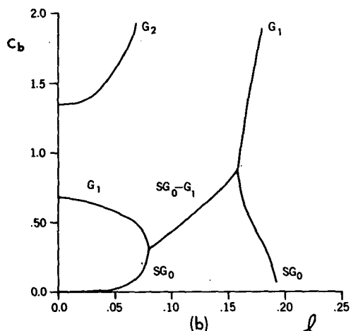
FIG. 12. (a) Nondimensional Reynolds stress conversion term C_r and (b) buoyancy conversion term of the shear-gravity mode SG_0 and the first two modified gravity modes, G_1 and G_2 , as a function of normalized horizontal wavenumber l for the case \xi_0/N_s = 0.8 and H/2a = 1 . See text for normalizations.
