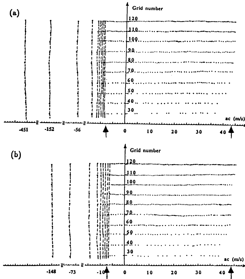
FIG. 2. Distribution of calculated spectra for different resolutions using observed zonal mean flow at 300 mb in October 1982. The ordinate gives the number of grids. The abscissa is the spectral values multiplied by the radius of the earth a . Arrows indicate maximum and minimum angular velocity of the basic flow multiplied by a . (a) For zonal wavenumber k = 1 . (b) For zonal wavenumber k = 2 .
