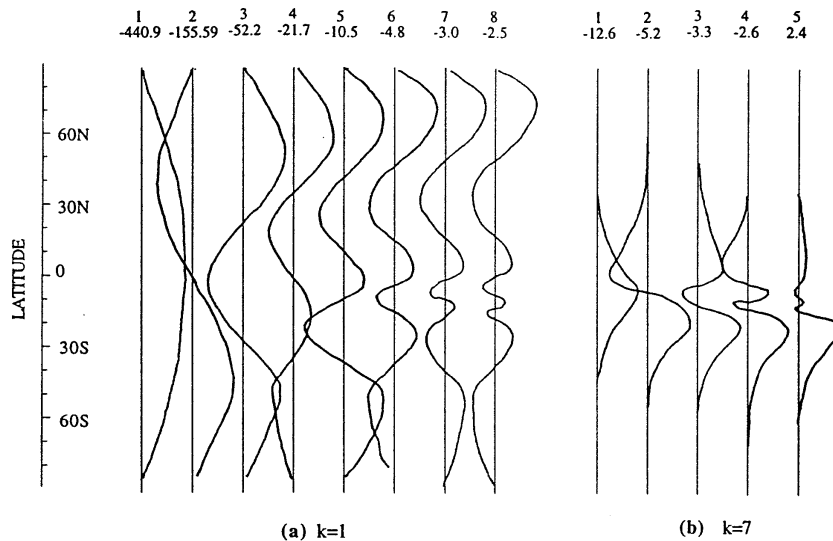
FIG. 4. Spectral functions of discrete spectra using January basic flow in Fig. 3a for zonal wavenumbers k = 1 (a) and k = 7 (b). Value listed above each function is the corresponding spectral value multiplied by the radius of the earth (unit in \text{m s}^{-1} ).
