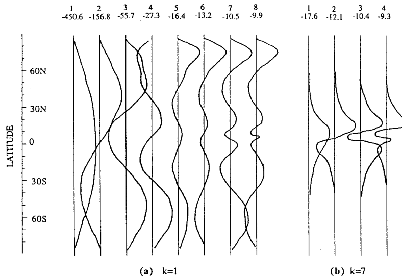
FIG. 5. Spectral functions of the neutral discrete spectra using the July basic flow in Fig. 3b for zonal wavenumbers k = 1 (a) and k = 7 (b). Value listed above each function is the corresponding spectral value multiplied by the radius of the earth (unit in m s^{-1} ).
