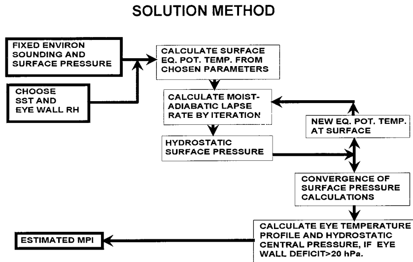
FIG. 3. Flow chart describing the solution method for estimating the MPI.
