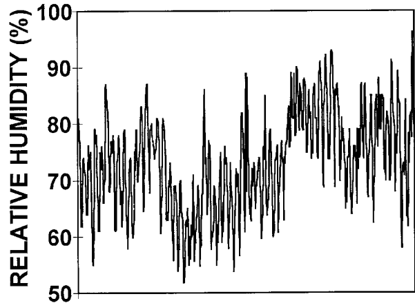
FIG. 1. Variation of surface relative humidity at Willis Island (a small coral cay, 500 km off the northeast Australian coast) for 3-h observations during January and February 1992.
