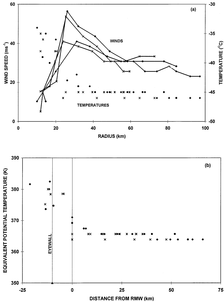
FIG. 10. Radial profiles at the 190–100-hPa level of (a) wind speed and temperature, and (b) equivalent potential temperature obtained from a NASA DC-8 reconnaissance of Supertyphoon Flo. The abscissa in (b) is relative to the RMW for each flight leg and the approximate position of the inner eyewall is shown.
