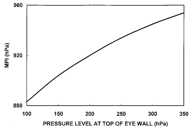
FIG. 9. Variation of MPI for changes in height of the eyewall based on the Willis Island January sounding.
