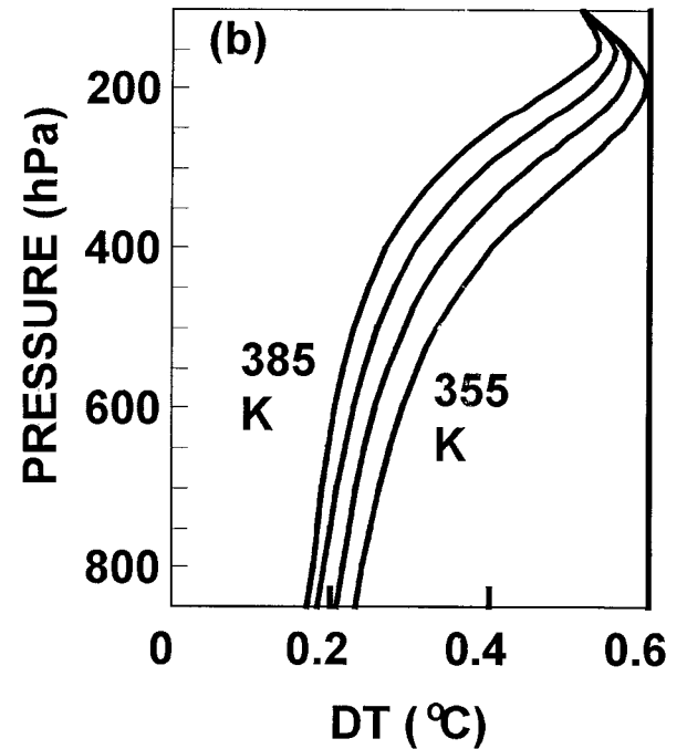
FIG. 5. Illustration of the reasons for convergence of the thermodynamic model: (a) Relative magnitudes of \partial\theta_{ES}/\partial P_s (dashed line, right axis) and \partial P_s/\partial\theta_{ES} (solid line, left axis) and their variation with surface pressure; (b) decreasing degree of warming between moist adiabats per K change of \theta_E for \theta_{ES} = 355, 365, 375, and 385 K (using Willis January sounding).
