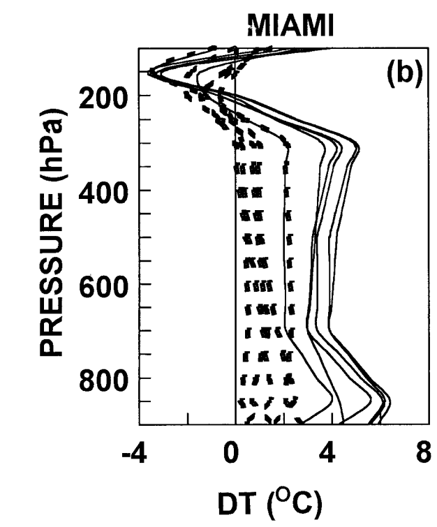
FIG. 14. Variations of monthly mean soundings from the month of coldest SST at (a) Willis Island and (b) Miami. Dashed lines indicate months where the MPI was below tropical cyclone strength.
