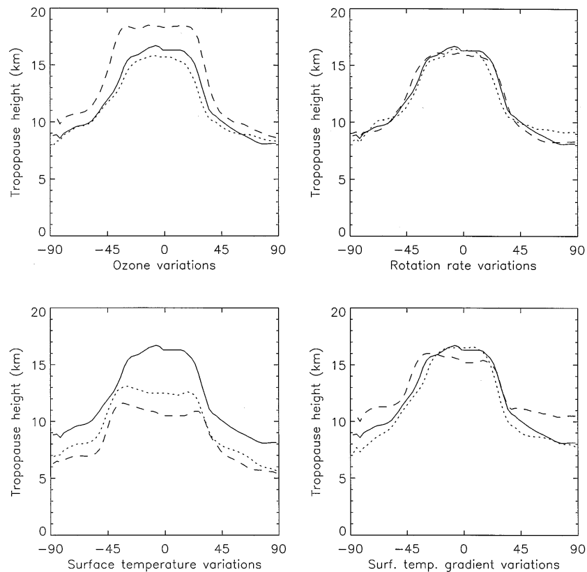
FIG. 4. Zonal mean 30-day mean tropopause height as a function of latitude for nine of the GCM experiments. In each panel the solid curve is for the control run, run 1. Upper left: dotted curve, run 2; dashed curve, run 3. Upper right: dotted curve, run 4; dashed curve, run 5. Lower left: dotted curve, run 6; dashed curve, run 7. Lower right: dotted curve, run 8; dashed curve, run 9.
