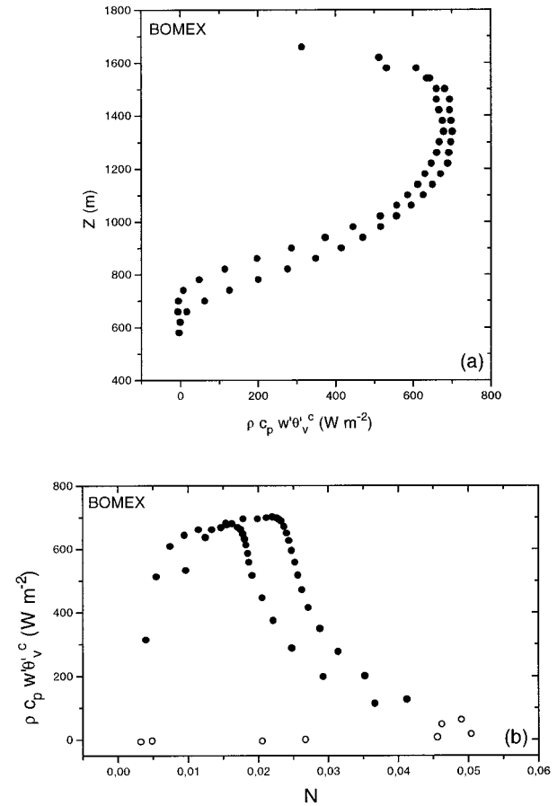
FIG. 1. The in-cloud buoyancy flux ( \text{W m}^{-2} ) as a function of height (a) and fractional cloudiness (b) from two 1-h time averages of a BOMEX simulation. In (b) the cloud base values are distinguished by open circles.
