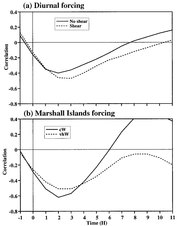
FIG. 11. As in Fig. 9b except for (a) diurnal forcing simulations and (b) Marshall Islands forcing simulations. See texts for further explanation.
