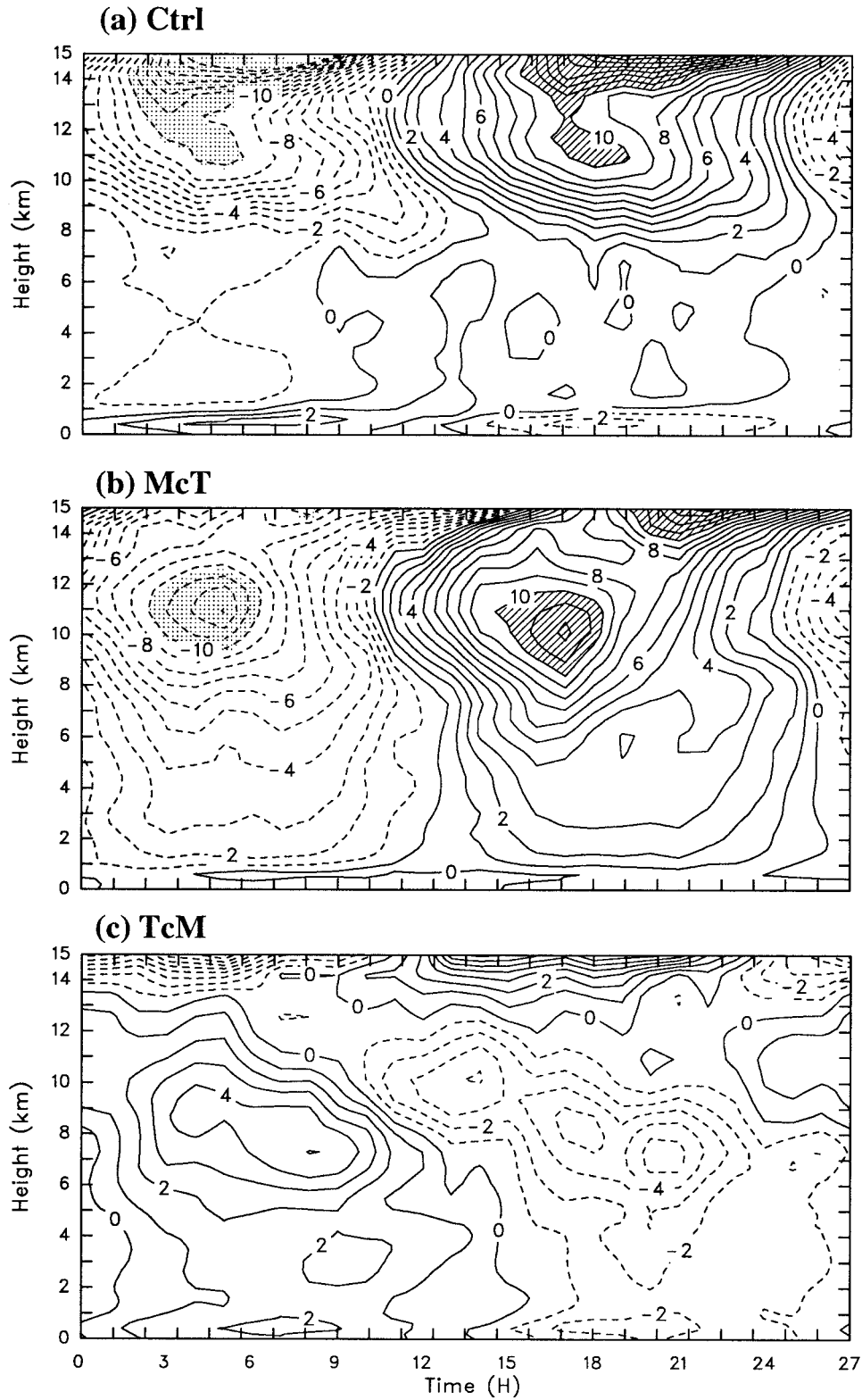
FIG. 7. As in Fig. 6 except for the ensemble mean of the relative deviation of water vapor mixing ratio (with respect to the mean value at each level of the respective simulation). The contour interval is 1%. Contours over 10% are hatched. Contours less than -10% are dotted.
