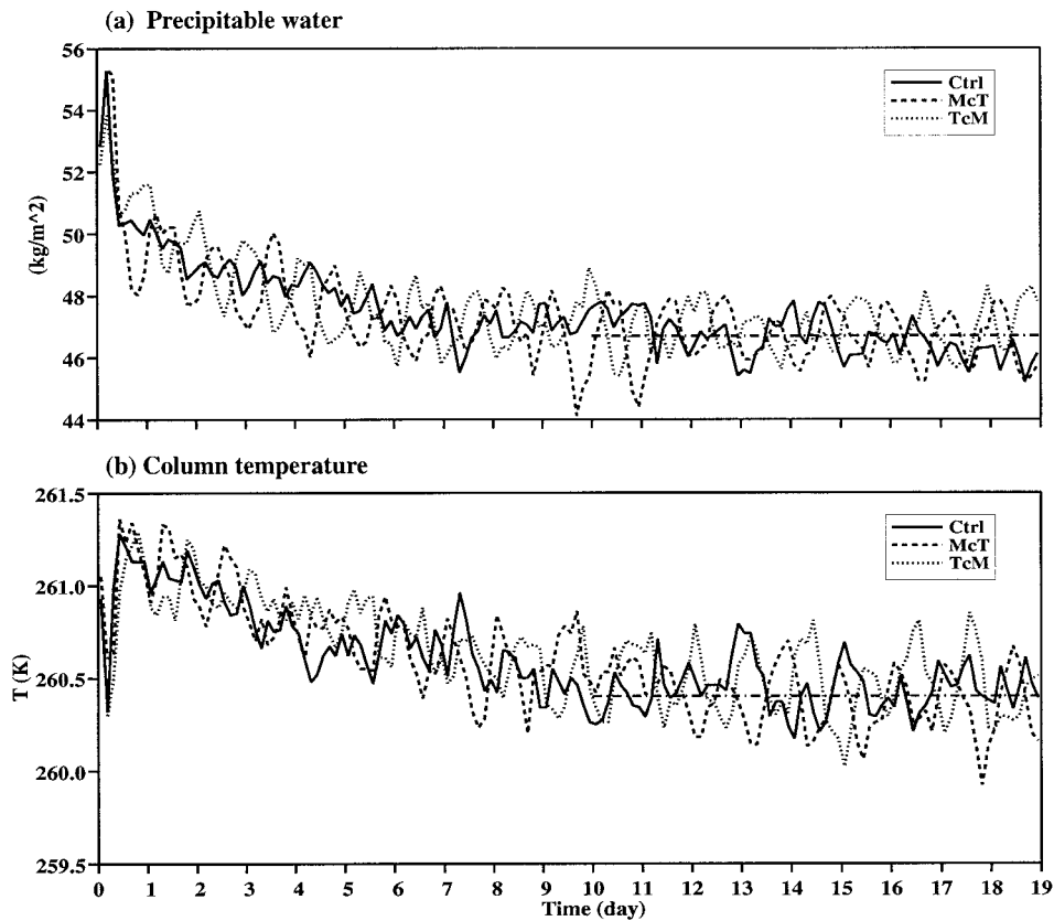
FIG. 1. Time sequence of the domain-averaged (a) precipitable water and (b) column temperature for simulations Ctrl, McT, and TcM. The horizontal dashed-dotted lines indicate the averaged value over the last nine days of the simulations.
