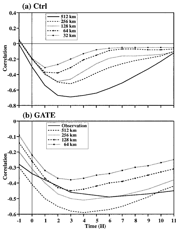
FIG. 10. Lag correlation coefficients between GCAPE and the surface precipitation rate as a function of horizontal averaging distances for (a) Ctrl and (b) GATE simulation and observation. Note the different scales in (a) and (b).
