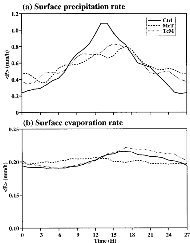
FIG. 4. As in Fig. 2 except for (a) surface precipitation rate and (b) surface evaporation rate for simulations Ctrl, McT, and TcM.
