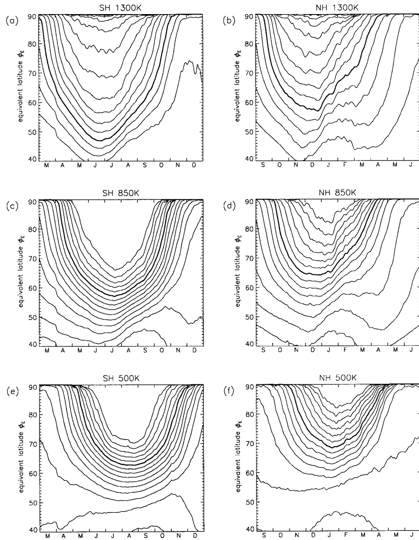
FIG. 2. Temporal evolution of climatological \phi_E for (left) Southern and (right) Northern Hemisphere at (upper) 1300 K, (middle) 850 K and (lower) 500 K. Contour interval is 2 PVU, and thick curves correspond to PV values in Table 1.
