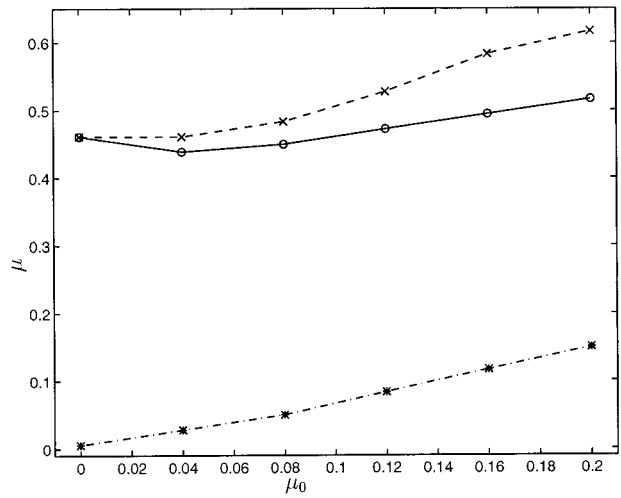
FIG. 3. The position of the easterly maximum (dash-dotted line with “*”), of the winter jet (solid line with “O”), and of the summer jet (dashed line with “X”). For compactness of the figure, the winter jet’s position is reflected about the equator and plotted in the same hemisphere as the summer jet.
