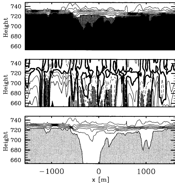
FIG. 2. Snapshots from an SMK-S-128 simulation at t=9000 s of \theta (upper panel, contours at 287.5, 288.0, 289.0, 290.0, 291.0, 292.0, 293.0, 294.0, 294.5 K), w (middle panel, contours at -1.00 , -0.50 , -0.25 , -0.10 , 0.00 , 0.10 , 0.25 , 0.50 , 1.00 , with negative contours dashed and zero contour thickened), and s (lower panel, contours at 0.05 , 0.20 , 0.35 , 0.50 , 0.65 , 0.80 , 0.95 , 0.98 , 1.00 ). Shading is applied to help accentuate features.
