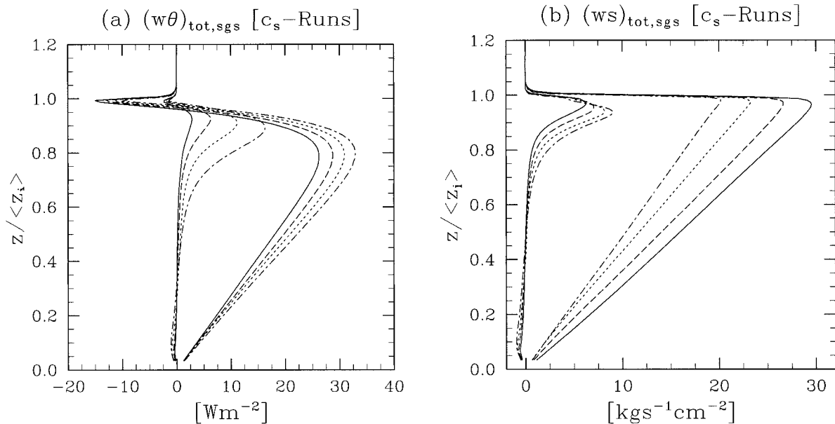
FIG. 7. Smoke cloud sensitivity of (a) theta and (b) smoke fluxes to changes in c_s for a suite of SMK-S-064 class simulations with c_s = 0.15 (solid), 0.23 (dashed), 0.35 (dotted), 0.53 (dash-dot).
