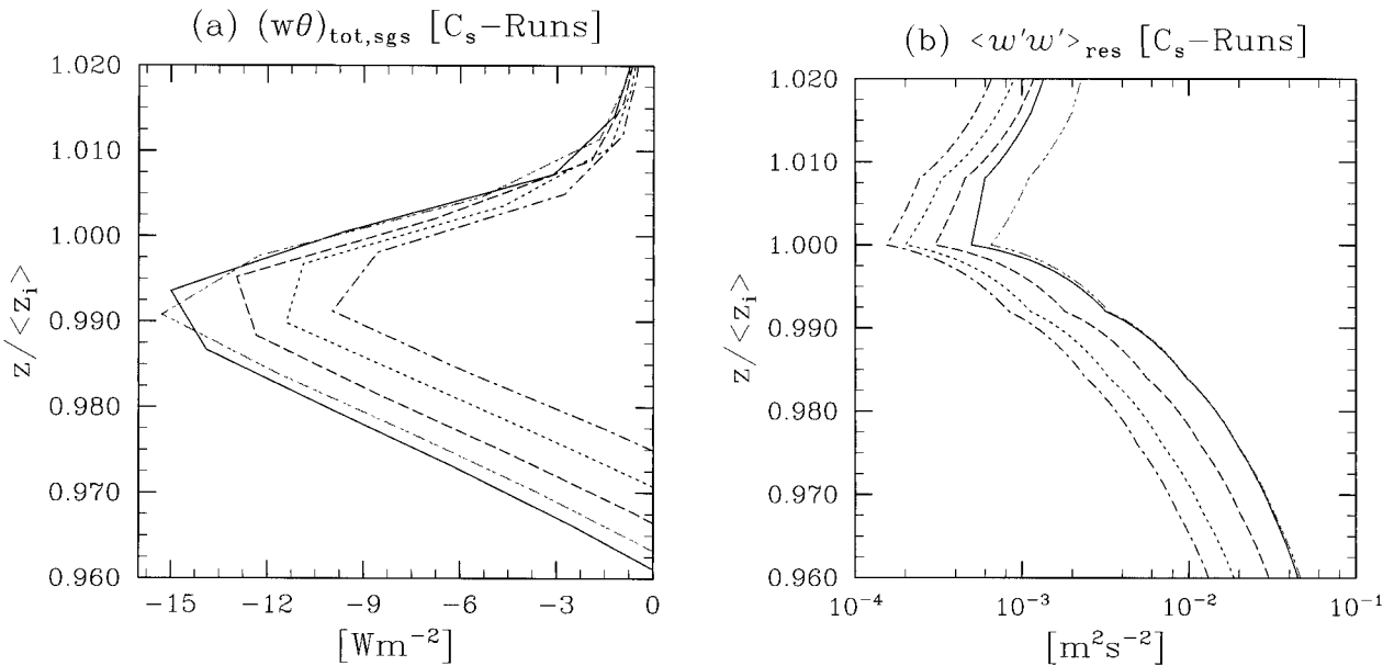
FIG. 15. (a) Entrainment heat fluxes and (b) vertical velocity variances from SMK-S-064 class simulations with c_s = 0.15 (solid), 0.23 (dashed), 0.35 (dotted), 0.53 (dash-dot), and an SMK-S-128 class simulation with c_s = 0.23 .
