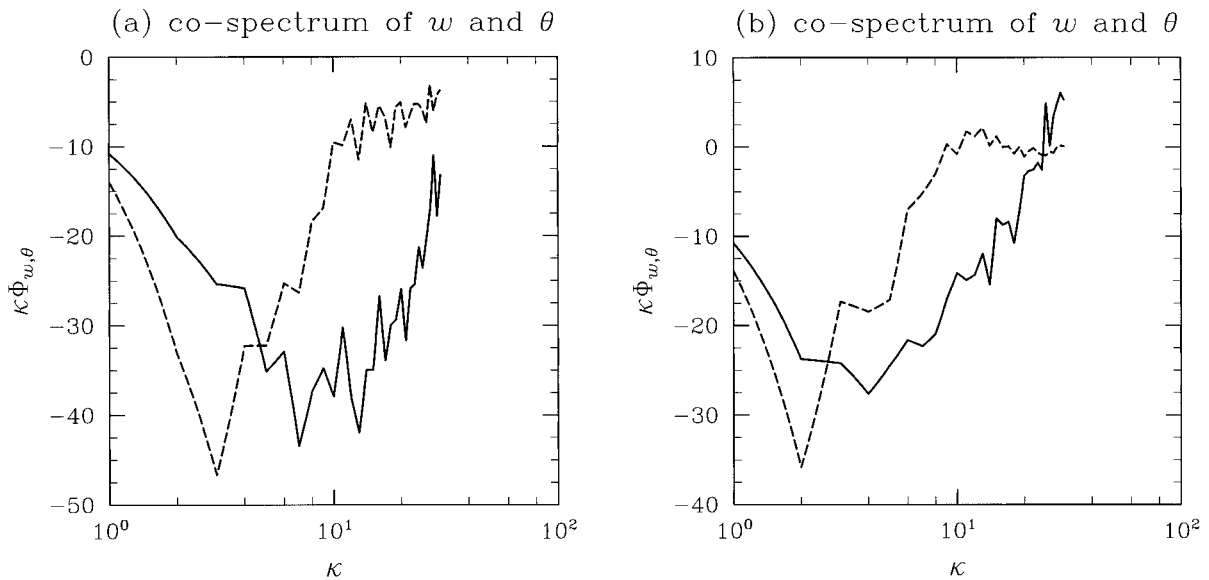
FIG. 9. Two-dimensional cospectra of w and \theta_* , where \theta_* is the value of \theta interpolated, on the basis of our advection algorithms, to a w point, and \kappa = (\kappa_w^2 + \kappa_\theta^2)^{1/2} . From SMK-S-064 class calculations. Solid line: c_s = 0.15 ; dashed line: c_s = 0.35 . Cospectra at (a) height where minimum buoyancy flux locates, and (b) 10 m (2 levels) below this point.
