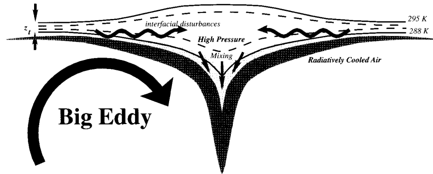
FIG. 4. Schematic figure of the nature of entrainment in a radiatively forced layer as represented by our LES. In part this figure represents the dynamics as we see them superimposed on a conditionally averaged view of the interface.
