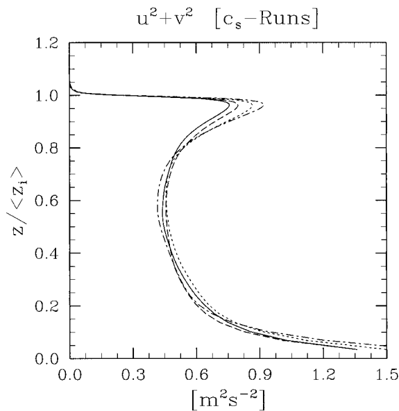
FIG. 11. Resolved variances in horizontal winds. Lines as in Fig. 7.
