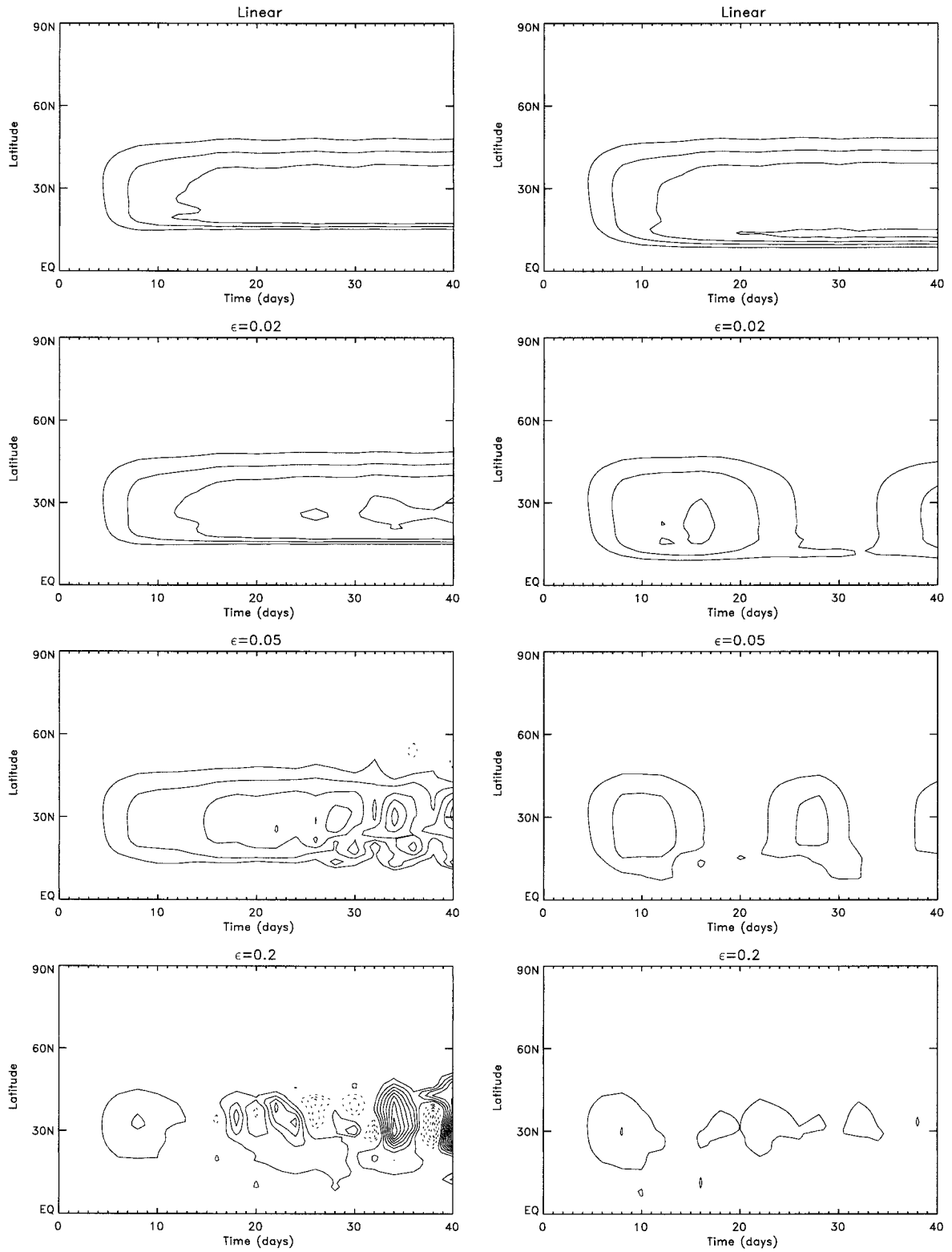
FIG. 4. Contour plot showing the evolution in latitude and time of the zonal mean meridional flux \bar{F}^{(\varphi)} in the wave-3 experiments. Left panels show the Hadley circulation case, and right panels the no-Hadley circulation case. The cases shown are the linear case ( \epsilon \rightarrow 0 ), \epsilon = 0.02, 0.05 , and 0.2 . Contour intervals are 0.005 \epsilon^2 \Omega^2 a^2 H . Negative contours are solid and positive contours dotted, and the zero contour is omitted.
