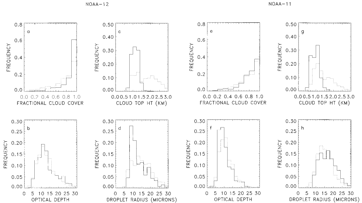
FIG. 7. Frequencies of fractional cloud cover, cloud-top altitude, 0.63- \mu\text{m} optical depth, and cloud droplet effective radius for 60-km regions within 50 km of a ship track head (solid line) and for regions that were more than 200 km from a ship track head (dashed line) for Jun 1994. The cloud altitudes, optical depths, and droplet radii were derived from the average radiances for the pixels found to be overcast within the 60-km regions. The observations are for ocean regions only. Morning NOAA-12 observations (a)–(d); afternoon NOAA-11 observations (e)–(h).
