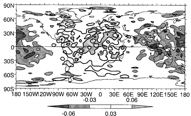
FIG. 12. As in Fig. 8 but for 10-hPa zonal wind. Contour interval is 0.03 \text{ m s}^{-1} ; negative contours are dotted and the zero contour is omitted. Shading is shown by the legend.
