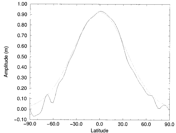
FIG. 11. As in Fig. 8 but for a meridional section of the zonal-wavenumber-1 component of the 500-hPa geopotential height anomaly through 25^{\circ}\text{W} (solid line). The meridional structure of a theoretical equatorial Kelvin wave with c = 340 \text{ m s}^{-1} is shown by the dotted line.
