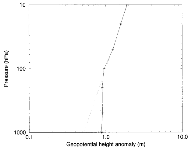
FIG. 10. Amplitude of the zonal-wavenumber-1 component of the regressed geopotential height anomalies averaged over 10^{\circ}\text{S} – 10^{\circ}\text{N} (solid line). The theoretical structure of an external mode with a surface amplitude scaled to match the observations in the stratosphere is shown by the dotted line. Both axes are plotted on a logarithmic scale.
