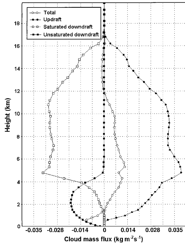
FIG. 10. 6-day (between 20 and 26 Dec) averaged cloud mass fluxes (CONTROL) in \text{kg m}^{-2} \text{s}^{-1} .
