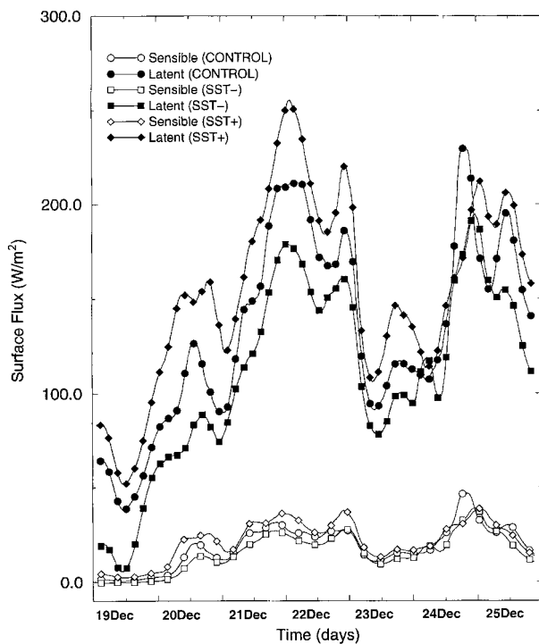
FIG. 16. Sensible and latent heat fluxes in CONTROL, SST-, and SST+, in W m^{-2} .
