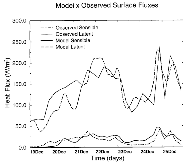
FIG. 5. Model vs observed surface heat fluxes, in \text{W m}^{-2} .
