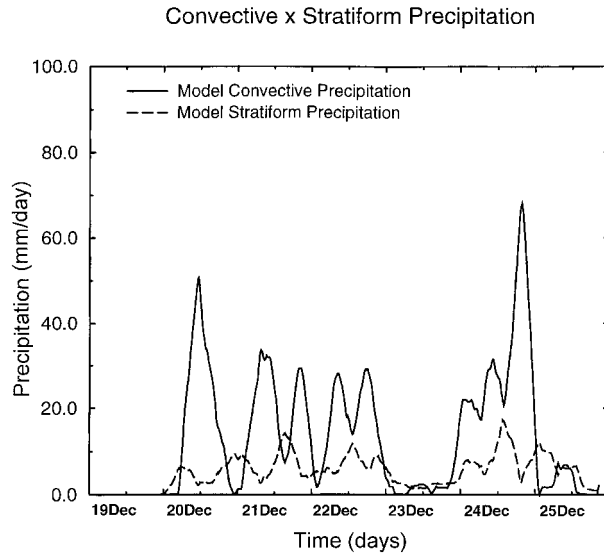
FIG. 9. Convective and stratiform precipitation, 3-h running domain average (CONTROL), in \text{mm day}^{-1} .
