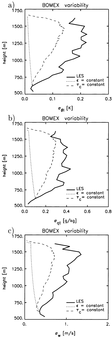
FIG. 8. The standard deviation of (a) \theta_i , (b) q_t , and (c) w of the core ensemble around the core average for BOMEX. The spikiness in the LES profile is caused by the fact that an instantaneous 3D field is used for the validation.
