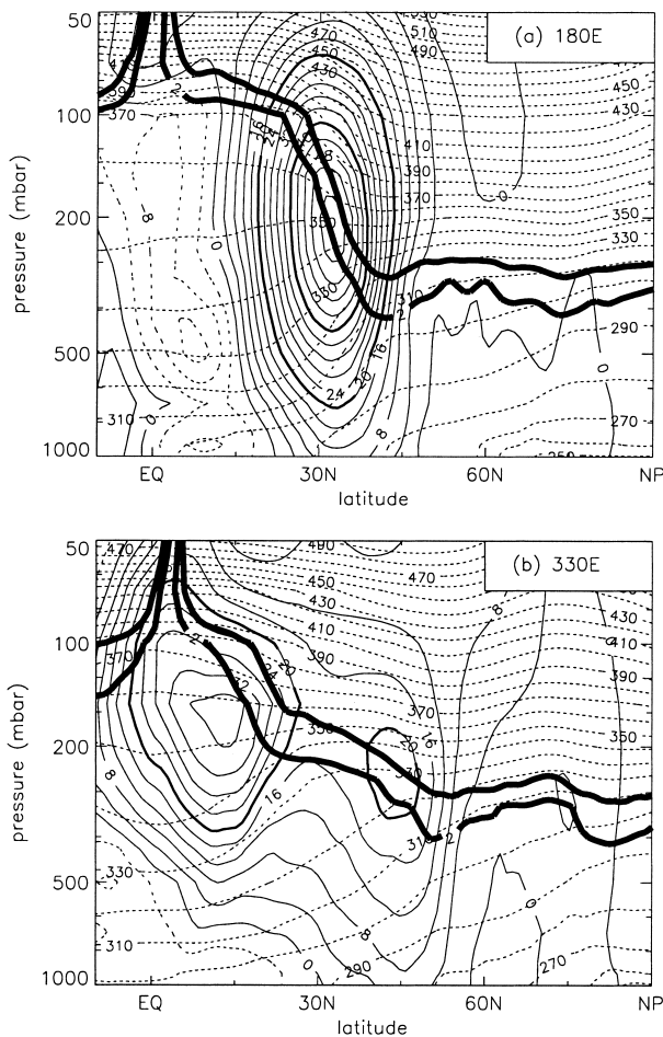
FIG. 11. Jan 1998 monthly mean meridional cross sections of zonal wind and potential temperature at (a) 180^\circ ; (b) 330^\circ E. Solid lines denote positive zonal wind, dotted lines denote negative zonal wind and potential temperature, and the thick lines denote the monthly mean 2- and 4-pvu potential vorticity contours.
