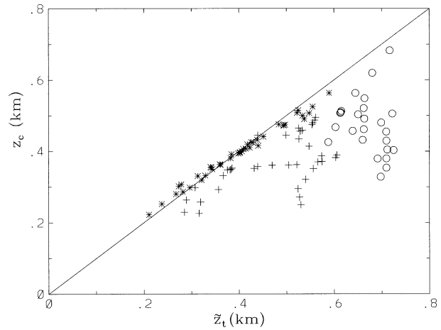
FIG. 12. Measured LES column cloud-base height z_c vs subcloud-layer height from CBL scaling \tilde{z}_t . Symbols as in Fig. 9.
