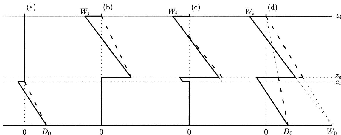
FIG. 2. Schematic buoyancy fluxes (solid line) and no-entrainment buoyancy fluxes (heavy dash) used in computing large-eddy entrainment efficiencies for different circulations and entrainment processes as described in the text: (a) \eta_{sc} , (b) \eta_c , (c) \eta_b , and (d) \eta_f .
