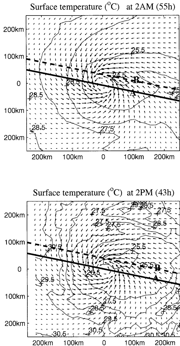
FIG. 10. Similar to Fig. 4 but for the experiments starting with land surface water conditions everywhere. The light-dashed line results from a case of an inhomogeneous surface of alternating 8- and 100-cm-deep water squares on a resolution of 1/6^\circ .
