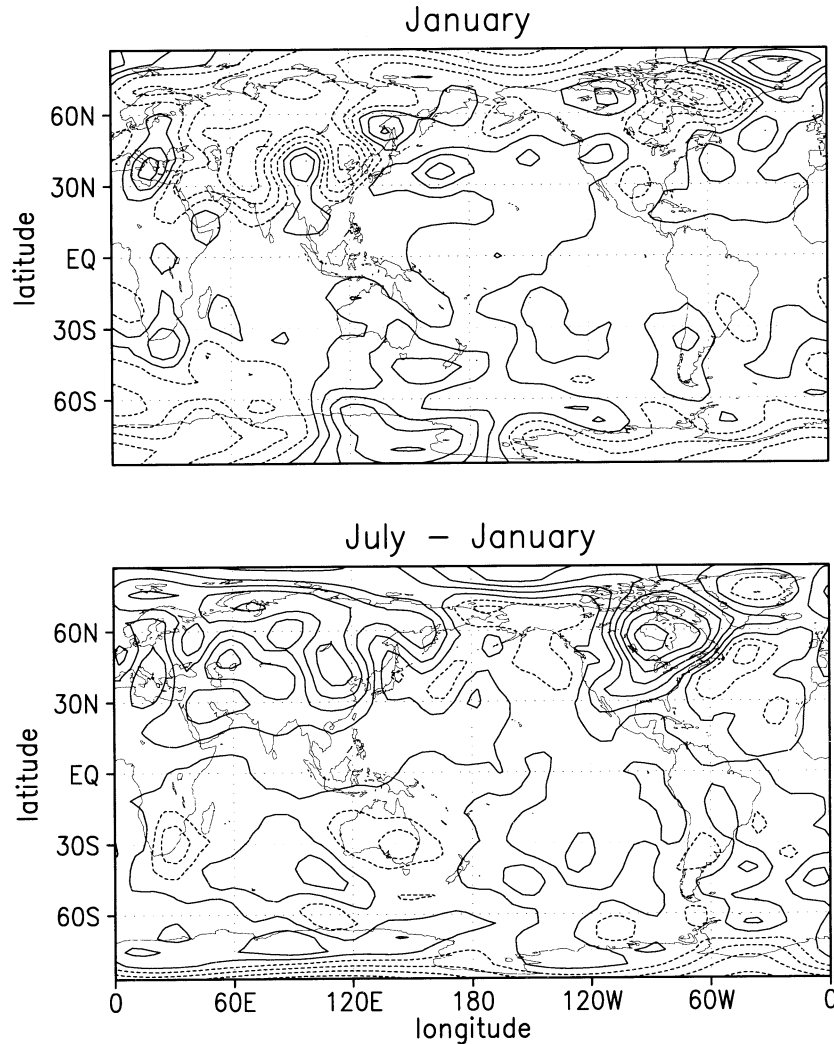
FIG. 5. Jan empirical forcing of the thermodynamic variable \tau at \sigma = 0.833 in (top) the semiempirical 500-EOF model, and (bottom) the difference between this and the corresponding field in Jul. Contour intervals are 0.02 \sqrt{\text{K day}^{-1}} . Negative values are dashed.
