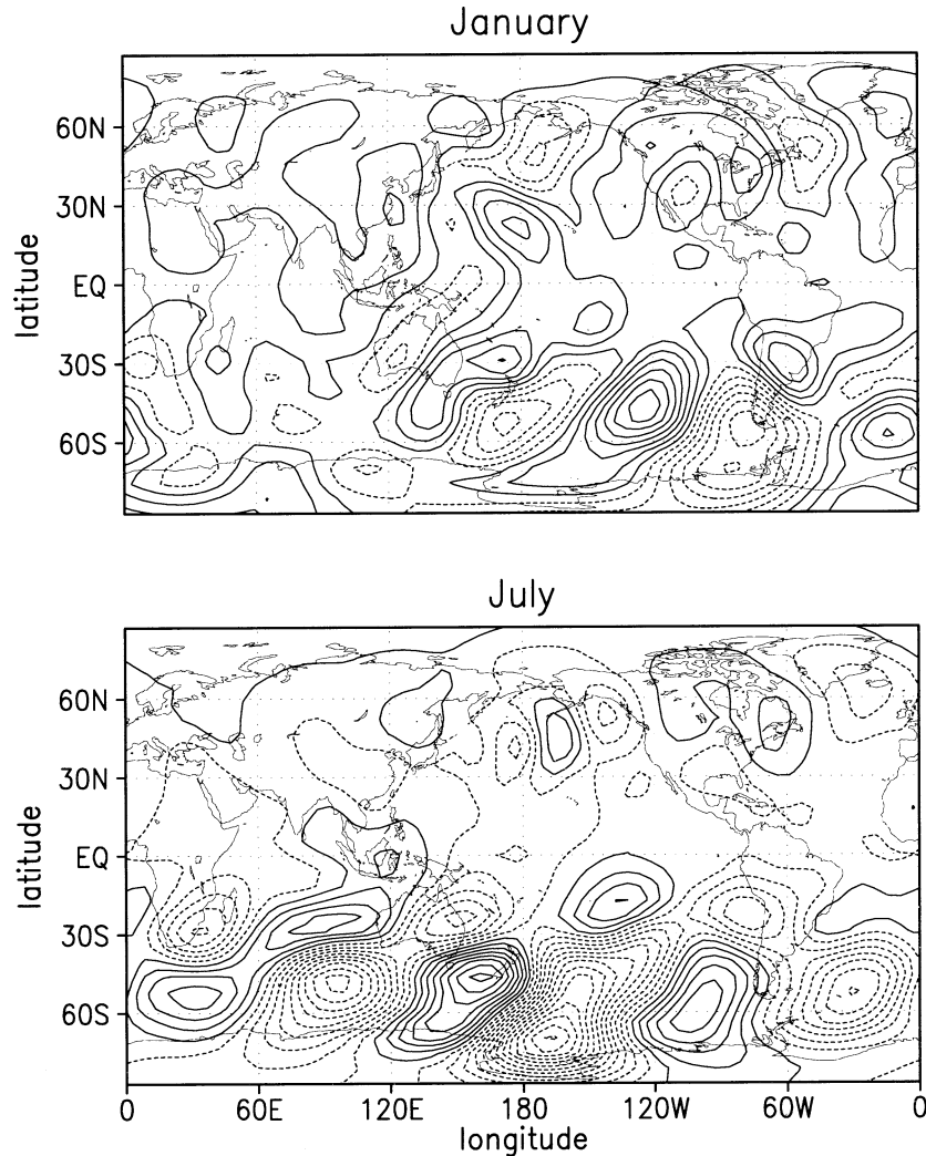
FIG. 7. As in Fig. 6, but for the 500-EOF model without empirical linear correction. The Jan growth factor is 9.46; that for Jul is 9.45.
