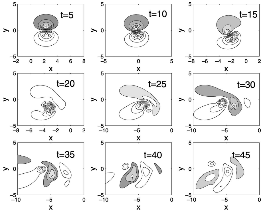
FIG. 9. Unstable evolution of a westward-moving modon perturbed by both the surface perturbation and bottom friction with \varepsilon = 0.05 and \mu = 0.01 . The modon parameters are as in Fig. 3.
