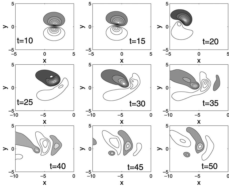
FIG. 5. Unstable evolution of a westward-moving modon subject to bottom friction with \varepsilon = 0.05 and \mu = 0.01 . The modon parameters are as in Fig. 3. The plots are the contour lines of the modon streamfunction.
