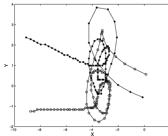
FIG. 2. As in Fig. 1, except the modon parameters are A = 1.0 , c = -0.95 , q = 0.973 , and k = 3.919 .
