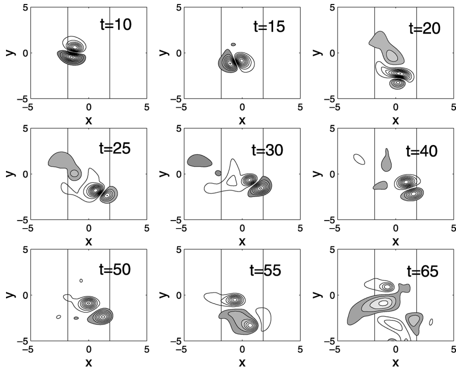
FIG. 8. Unstable evolution of an eastward-moving modon broken down by the topographic forcing with \epsilon = 0 , \mu = 0 , and h_0 = 1.30 . The curves are the contour lines of the modon streamfunction and the ridge is located between the vertical solid lines. The modon parameters are the same as in Fig. 7.
