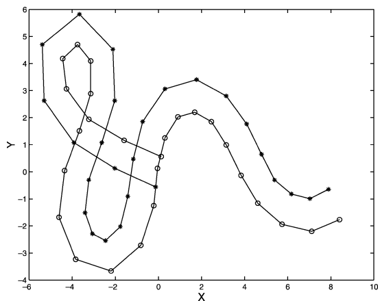
FIG. 1. Unstable evolution of a westward-moving modon tilted initially by an angle of \pi/10 . Curve with stars (topmost curve on rightside) is the trajectory of the anticyclone and curve with circles is the trajectory of the cyclone. The initial position of the center of the modon is located at x = 0 . The modon parameters are A = 1.0 , c = -1.95 , q = 1.220 , and k = 3.955 .
