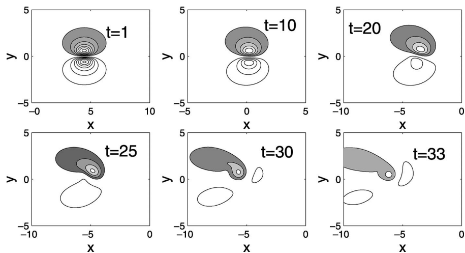
FIG. 10. As in Fig. 9, except \mu = 0.05 .
