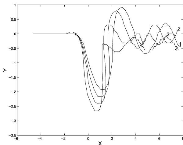
FIG. 7. Stable evolution of an eastward-moving modon that survives the topographic forcing with \varepsilon = 0 and \mu = 0 . The curves are the trajectories of the centers of the modons. The curves 1, 2, 3, and 4 represent the cases where h_0 = 0.9, 1.0, 1.1, 1.2 , respectively. The modon parameters are A = 1.0, c = 0.4, q = 2.121 , and k = 4.091 .
