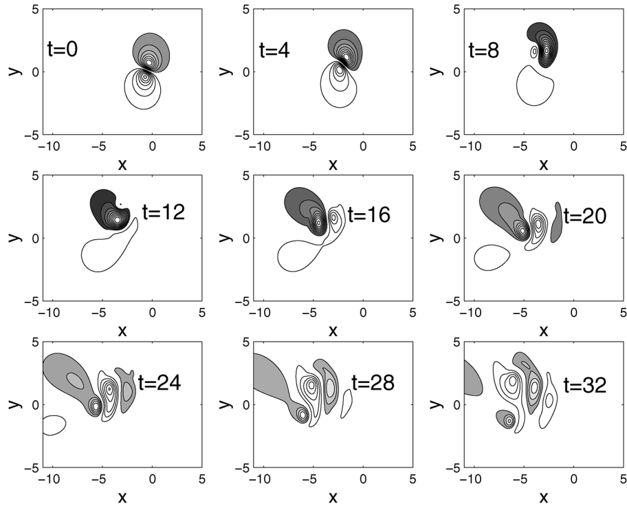
FIG. 3. Unstable evolution of a westward-moving modon tilted initially by an angle of \pi/10 . Curves in the plot are the contour lines of the modon streamfunction. The interval of the contour lines is 0.1 and the zero contour line has been omitted for clarity. Contour lines are shaded to represent the anticyclone while contour lines with no shading represent the cyclone (the same is true in the following figures). The modon parameters are A = 1.0 , c = -0.55 , q = 0.4264 , and k = 3.853 .
