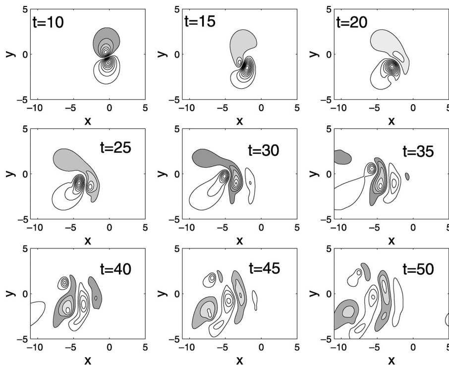
FIG. 4. Unstable evolution of a westward-moving modon perturbed by the upper-surface perturbation with \varepsilon = 0.05 . The modon parameters are the same as in Fig. 3.
