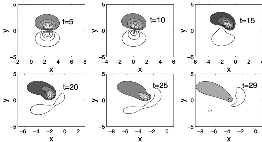
FIG. 6. As in Fig. 5, except \mu = 0.05 .
