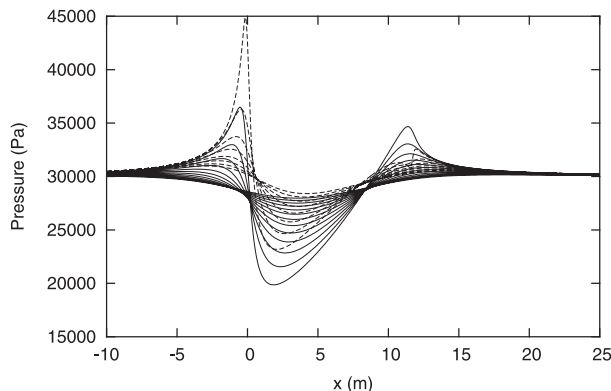
FIG. 4. Pressure variation on the trajectories of Fig. 3. Solid lines correspond to trajectories above the wing; dashed lines refer to trajectories below the wing. The vertical distance of the streamlines in the undisturbed farfield is about 60 cm. Note that the pressure drop is stronger above than below the wing. The resulting upward force carries the aircraft. Ambient pressure is 300 hPa.
