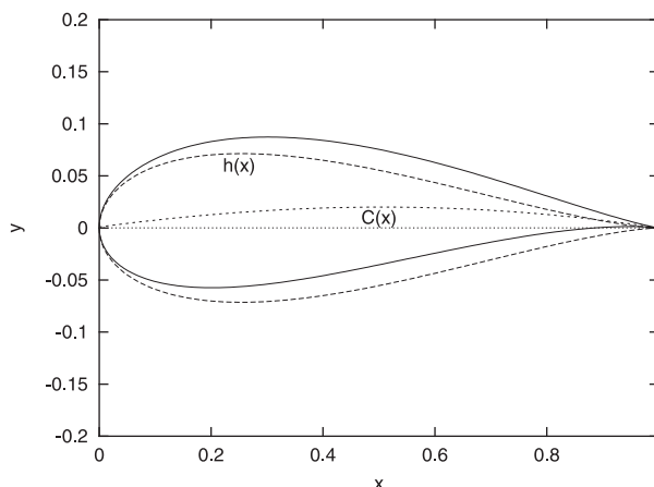
FIG. 2. Geometry of a Joukowski airfoil with x_c = 0.11 , y_c = 0.04 . The solid line is the wing surface. The surface can mathematically be represented as the sum of the surface of a symmetric wing (long dashed) plus a camber curve C(x) (short dashed); h(x) is the upper surface of the symmetric wing. Note that the y axis has been expanded for easier viewing.
