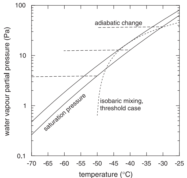
FIG. 8. A T - \log e phase diagram showing saturation lines for water and ice, together with some sample adiabatic lines and the critical mixing trajectory for exhaust contrail formation according to the Schmidt–Appleman theory. In this frame the adiabatic lines are straight lines with constant distance, but the saturation curves are slightly concave.
