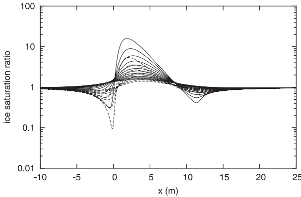
FIG. 6. As in Fig. 4, but for the ice saturation ratio. Ambient saturation ratio is 1.
