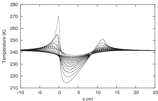
FIG. 5. As in Fig. 4, but for the temperatures. Ambient temperature is 241 K.
