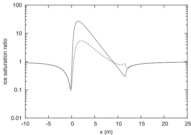
FIG. 7. As in Fig. 6, but for a pair of streamlines that encounter the leading edge of the wing at a vertical distance of 45 cm below (dashed line) and 45 cm above (solid line). Note that the curves are close to each other at the frontal stagnation point but far apart on the wing, with much higher supersaturation on the upper than the lower surface.
