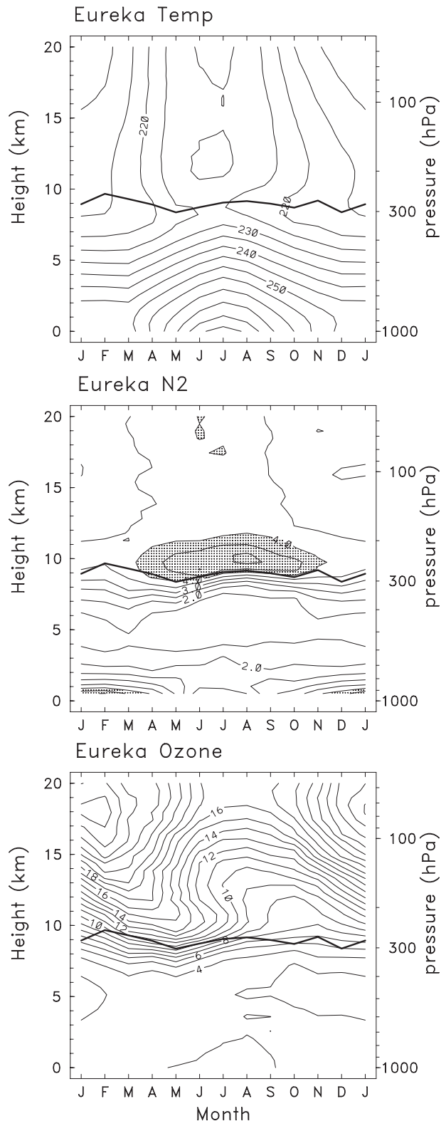
FIG. 6. Climatological seasonal variation of (a) temperature (K), (b) N^2 ( 10^{-4} \text{ s}^{-2} ), and (c) ozone density ( \text{DU km}^{-1} ) for the Arctic (from Eureka observations over 1992–2007). The tropopause is denoted as a thick line in each panel.
