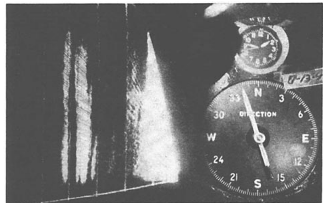
FIG. 5. Example of bright band development near an active thunderstorm.
