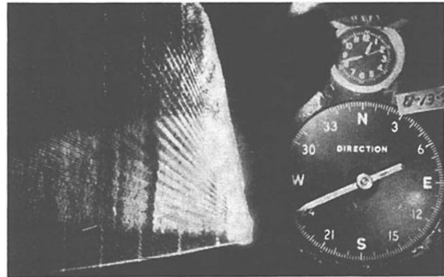
FIG. 4. Example of bright band in the rear of a thunderstorm.
