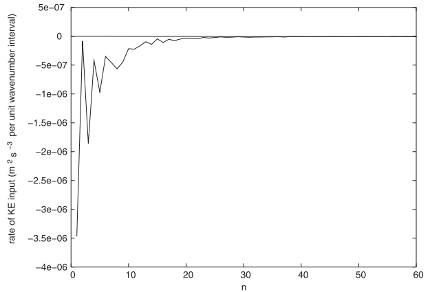
FIG. 5. Sum of S_{RWS}(n) and S_{TIP}(n) (denoted TIP).
