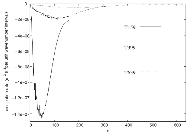
FIG. 8. Spectral distribution of KE dissipation rate (rotational flow only) at about 250 hPa for three model resolutions (T159, T399, and T639).
