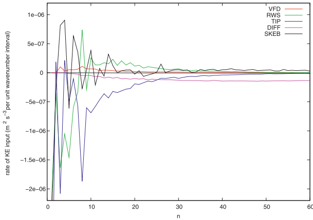
FIG. 4. As in Fig. 3, except zoomed in on the wavenumber range 0 \leq n \leq 60 for clarity.
