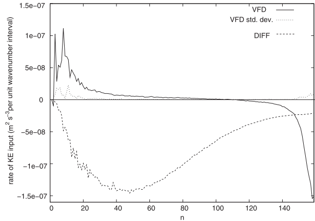
FIG. 1. Plot of S_{VFD} (solid), standard deviation of the daily mean about the 30-day mean (dotted line), and the dissipation rate due to horizontal diffusion (DIFF; dashed line) vs n at approximately 250 hPa.
