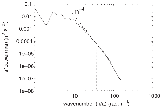
FIG. 2. Rotational kinetic energy spectrum in a T159 forecast showing the steep roll off beyond n = 40 where the slope approximates n^{-4} .
