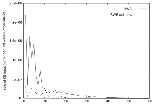
FIG. 7. |S_{RWS}| (solid) and standard deviation of S_{RWS} (dashed) vs n .
