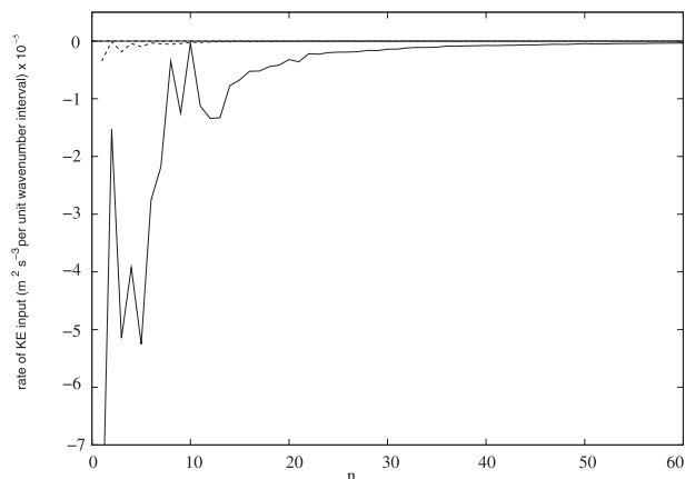
FIG. 6. Spectral distribution of KE dissipation due to model parameterization (solid) with the sum of S_{RWS} and S_{TIP} shown for reference (dashed). Note that units are m^2 s^{-3} \times 10^{-5} .
