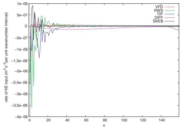
FIG. 3. Rate of kinetic energy input vs wavenumber for the individual components: S_{VFD}(n) , S_{RWS}(n) , and S_{TIP}(n) together with the energy sink due to horizontal diffusion and the energy source due to the SKEB scheme.
