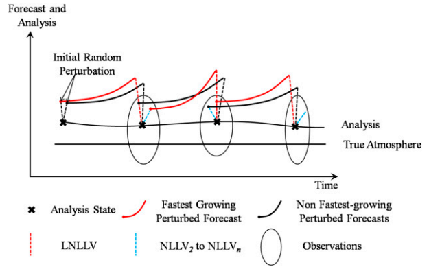
FIG. 2. Schematic representation of the analysis cycle and the creation of NLLVs. In each analysis cycle, the analysis states are updated by combining the background forecasts (black dashed curve) and the observations (open circle). NLLVs are attained to capture the fastest-growing components of the analysis errors. A group of initial random perturbations are added to the initial analysis state and integrated to the end of a breeding cycle similar to the background forecast in analysis cycles. The red solid curve represents the fastest-growing perturbed forecast during each cycle and the black solid curves represent other perturbed forecasts from the second to the n th fastest. The resulting perturbations between the analysis and the perturbed forecasts are then rearranged according to their growth rates during the last cycle. The direction of the fastest-growing mode (LNLLV, red dashed line) is kept, and the other directions (black dashed lines) are orthogonalized successively to acquire NLLV 2 to NLLV n (blue dashed line). Then these perturbations are rescaled to the same size as the initial perturbations. This process is repeated for several cycles to obtain effective NLLVs.
