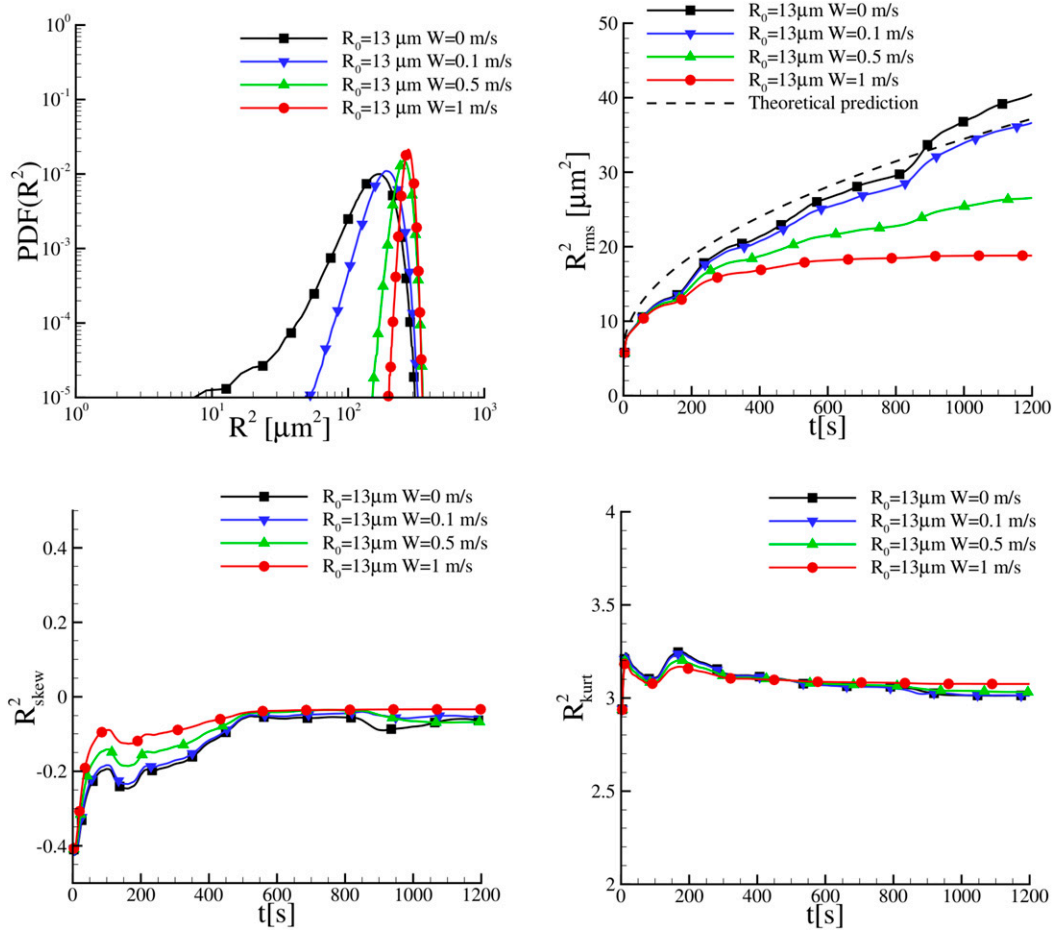
FIG. 3. (top left) Squared droplet radii pdf after 20 min of simulation for the largest droplets. Temporal evolution of squared droplet radius (top right) standard deviation, (bottom left) skewness, and (bottom right) kurtosis for the largest droplets.
