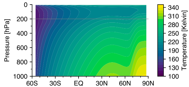
FIG. 2. Temperature as a function of latitude and pressure from the solstitial RCE simulation, as indicated in the color bar. The gray line at 200 hPa indicates the level at which the temperature is used to compute the gradient-balanced wind.
