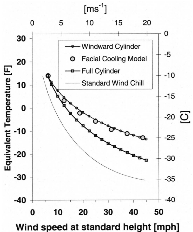
FIG. 2. Wind chill equivalent temperatures calculated at an air temperature of 14^\circ\text{F} ( -10^\circ\text{C} ).
