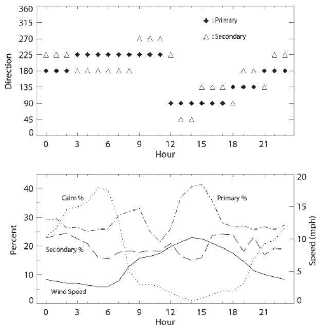
FIG. 2. Hourly wind normals for Daytona Beach, Florida, on 20 Jul (1981–2010). In the upper panel, the filled diamonds and open triangles indicate the wind sectors accounting for the highest two percentages of all noncalm wind events. In the lower panel, time series throughout the day are plotted for average wind speed (solid line), percentages associated with primary (dash-dot line) and secondary (long dash line) directions, and calm (dotted line) events.
