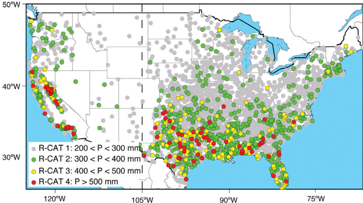
Fig. 3. Maximum 3-day precipitation totals at 5,877 COOP stations in the conterminous United States during 1950–2008. Each site used here had to have at least 30 years of records.
