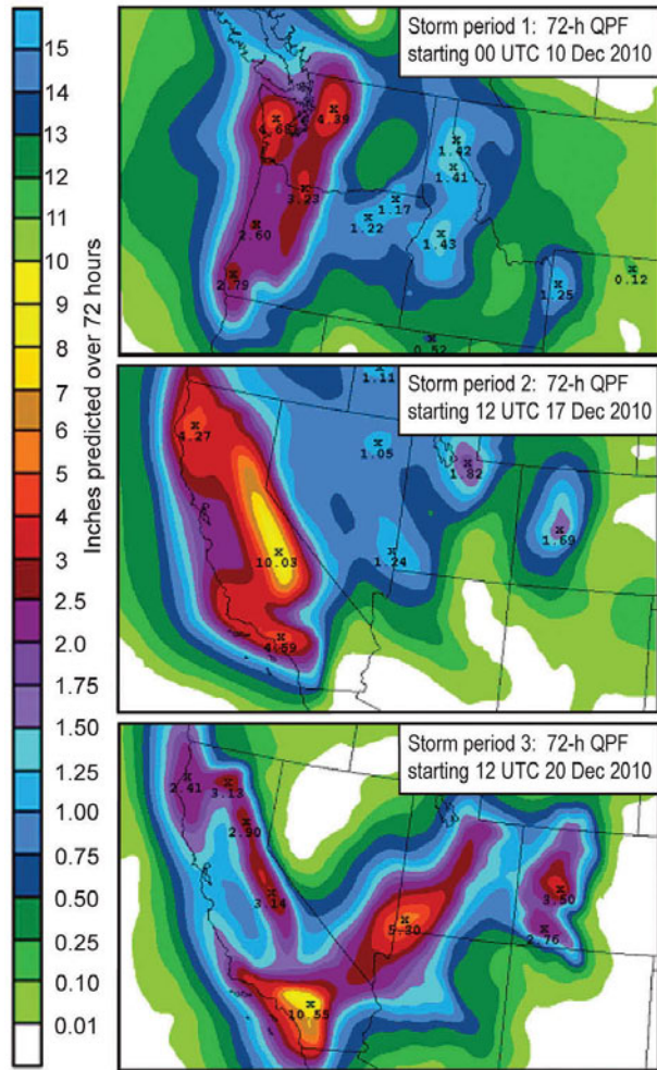
FIG. 6. HPC 3-day precipitation forecasts (in inches). These forecasts were issued at (top) 9 Dec 2010 at 1350 PST for 0000 UTC 10 Dec to 0000 UTC 13 Dec; (middle) 17 Dec 2010 at 0151 PST for 1200 UTC 17 Dec to 1200 UTC 20 Dec; and (bottom) 20 Dec 2010 at 0202 PST for 1200 UTC 20 Dec to 1200 UTC 23 Dec.
