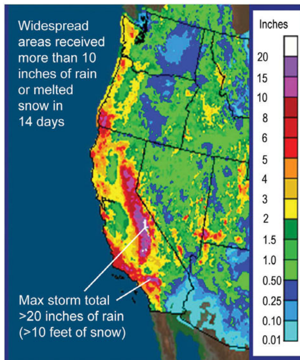
FIG. 1. 14-day observed precipitation in the western United States (courtesy of NWS Advanced Hydrologic Prediction Service).
