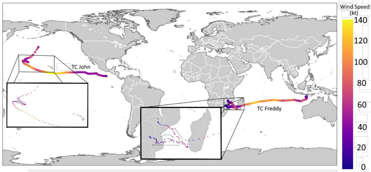
Fig. 1. Best tracks of TC John (1994) and TC Freddy (2023) with wind speed in color. Inset maps show the retrogression motion occurring in both TCs.
