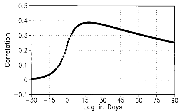
FIG. 16. Theoretical lag cross-correlation curve between the atmosphere and SST, according to the stochastic atmospheric forcing model of Frankignoul and Hasselmann (1977), for e -folding time-scales of (8 \text{ days})^{-1} for the atmospheric forcing and (5 \text{ months})^{-1} for SST. Note that the maximum cross correlation occurs at lag +18 days.
