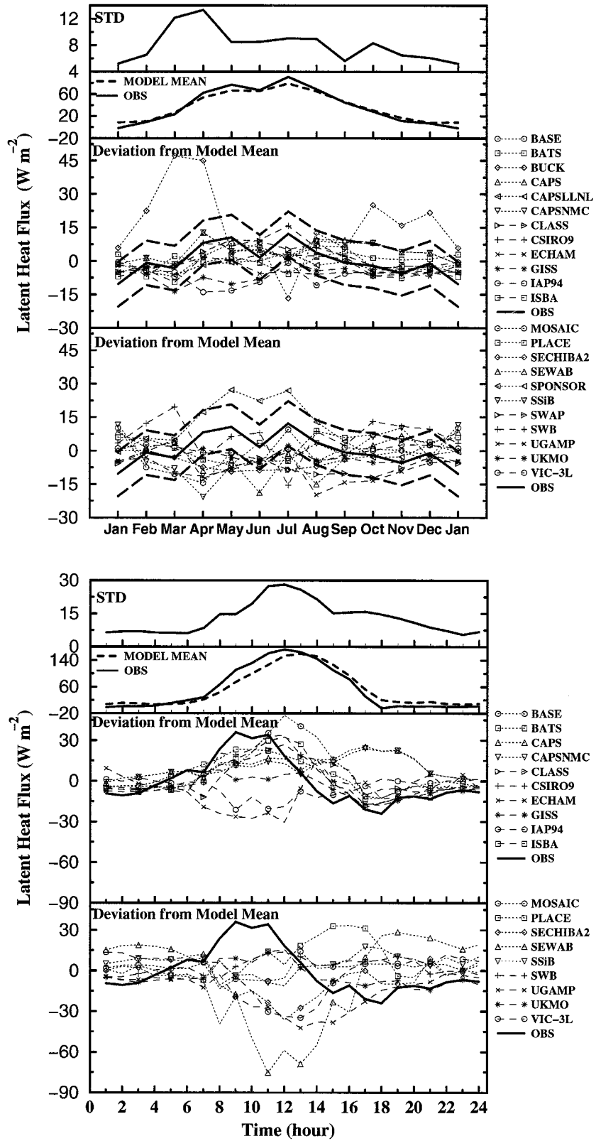
FIG. 6. As in Fig. 3 except for latent heat flux ( \text{W m}^{-2} ). The two thick dashed lines in panels 3 and 4 represent the estimated \pm 10 \text{ W m}^{-2} observation errors.
