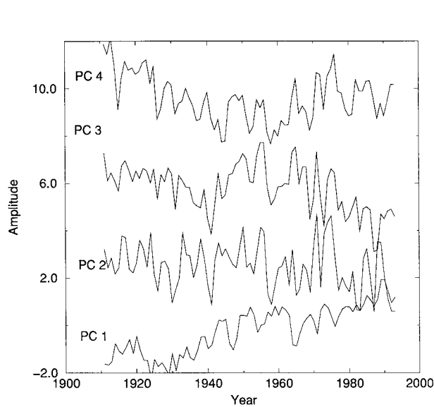
FIG. 9. Rotated principal component time series, normalized by their respective standard deviations. Each series is displaced along the ordinate for legibility.
