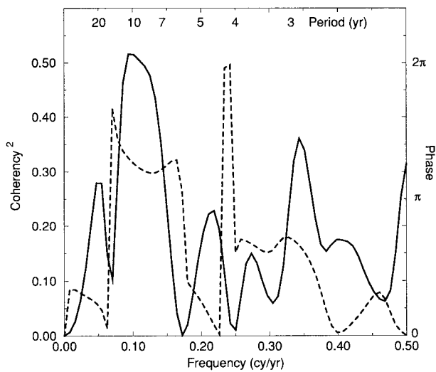
FIG. 13. Squared coherency (solid line) and phase (dashed) of a cross-spectral analysis of the Paraguay–Paraná time series ( x ) and an index of SST over the tropical North Atlantic ( y ). The latter was obtained by averaging SST anomalies over the region 0^{\circ} – 20^{\circ} N and 60^{\circ} W– 0^{\circ} . A Tukey window of 20 yr was used, giving a 95% confidence level for the squared coherency of 0.486.
