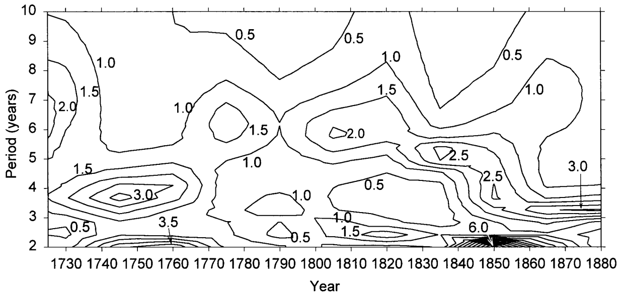
FIG. 10. Evolutionary spectrum of the southwestern United States fire-scar time series, 1700–1900. Maximum entropy spectral analysis (Marple 1987) was used to compute spectra for frequency bands 0.5–3.3 cycles \text{yr}^{-1} (2–10-yr periods) for 30-yr episodes overlapped by 15 yr. Contours of spectral estimates in standardized units versus time are shown. Biennial oscillations (i.e., circa 2-yr period) and circa 3–4-yr oscillations dominated during the midcentury periods, but were weak during the late 1700s to early 1800s when 5–7-yr oscillations become more important.
