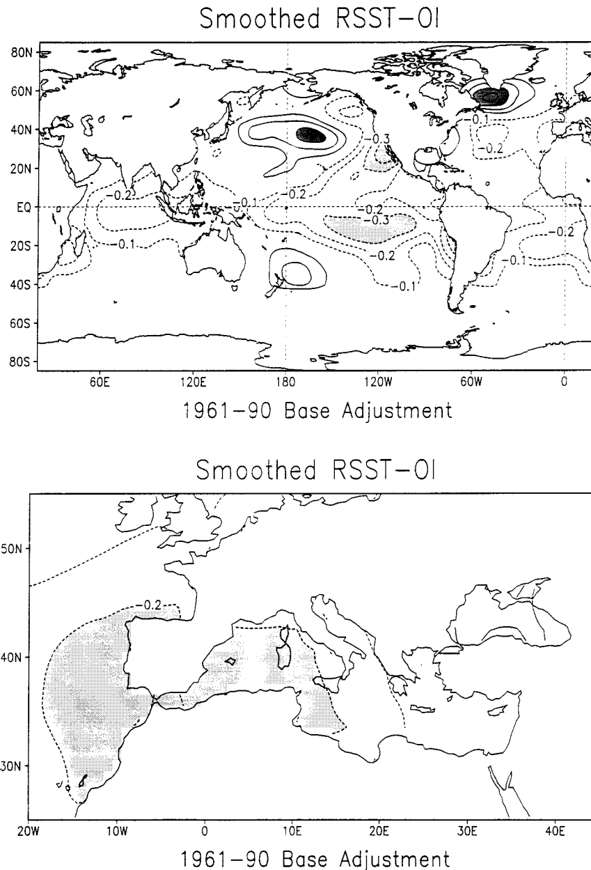
FIG. 1. Annual average of the adjustment for the OI climatology. Contour interval is 0.1^{\circ}\text{C} , the zero contour is omitted. In (a) values less than -0.3^{\circ}\text{C} and greater than 0.3^{\circ}\text{C} are shaded, and in (b) values less than -0.2^{\circ}\text{C} and greater than 0.2^{\circ}\text{C} are shaded.
