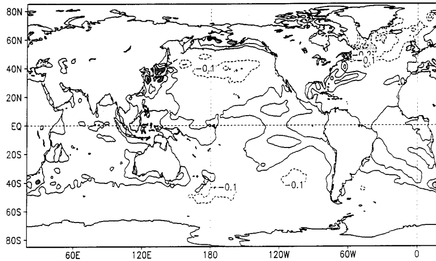
FIG. 2. Annual average difference in the climatologies, 1961–90 climatology minus the 1950–79 climatology of RS. Contour interval is 0.1^{\circ}\text{C} , the zero contour is omitted and values less than -0.3^{\circ}\text{C} and greater than 0.3^{\circ}\text{C} are shaded.
