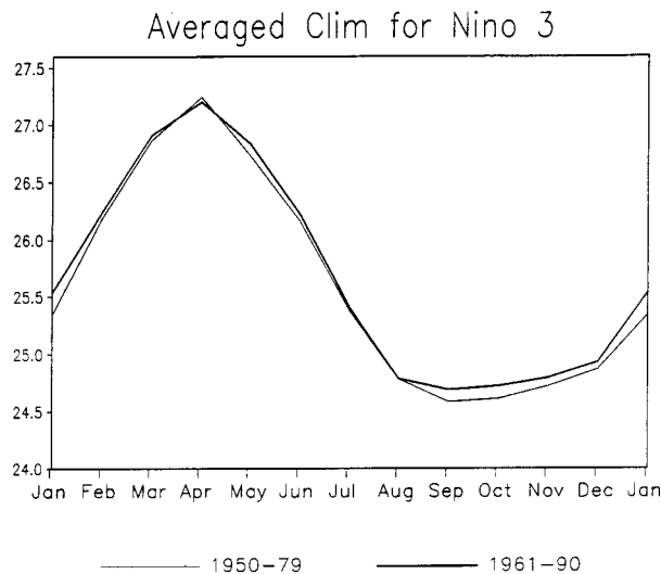
FIG. 3. Annual cycle of the 1961–90 climatology and the 1950–79 climatology, averaged in the Niño3 region ( 5^{\circ}\text{S} – 5^{\circ}\text{N} , 150^{\circ} – 90^{\circ}\text{W} ), in ^{\circ}\text{C} .
