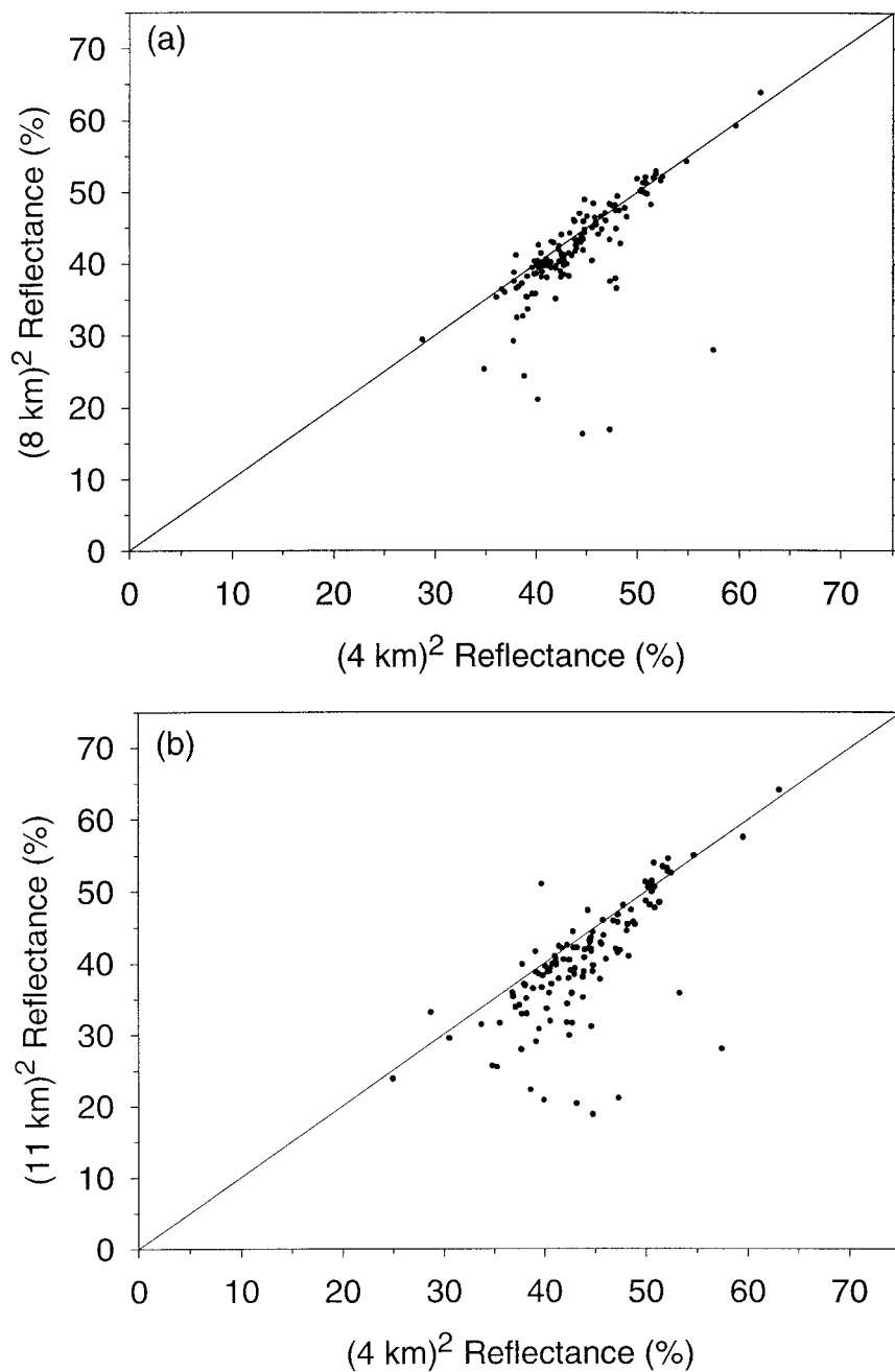
FIG. 1. Degraded- and full-resolution overcast nadir reflectances for degraded pixel resolutions of (a) 8 km and (b) 11 km. Full-resolution pixel is 4 km (GAC). Each point represents an average reflectance over the same scene (one scene per day) at the two resolutions. Included are all images with \mu_o > 0.4 (133 cases).
