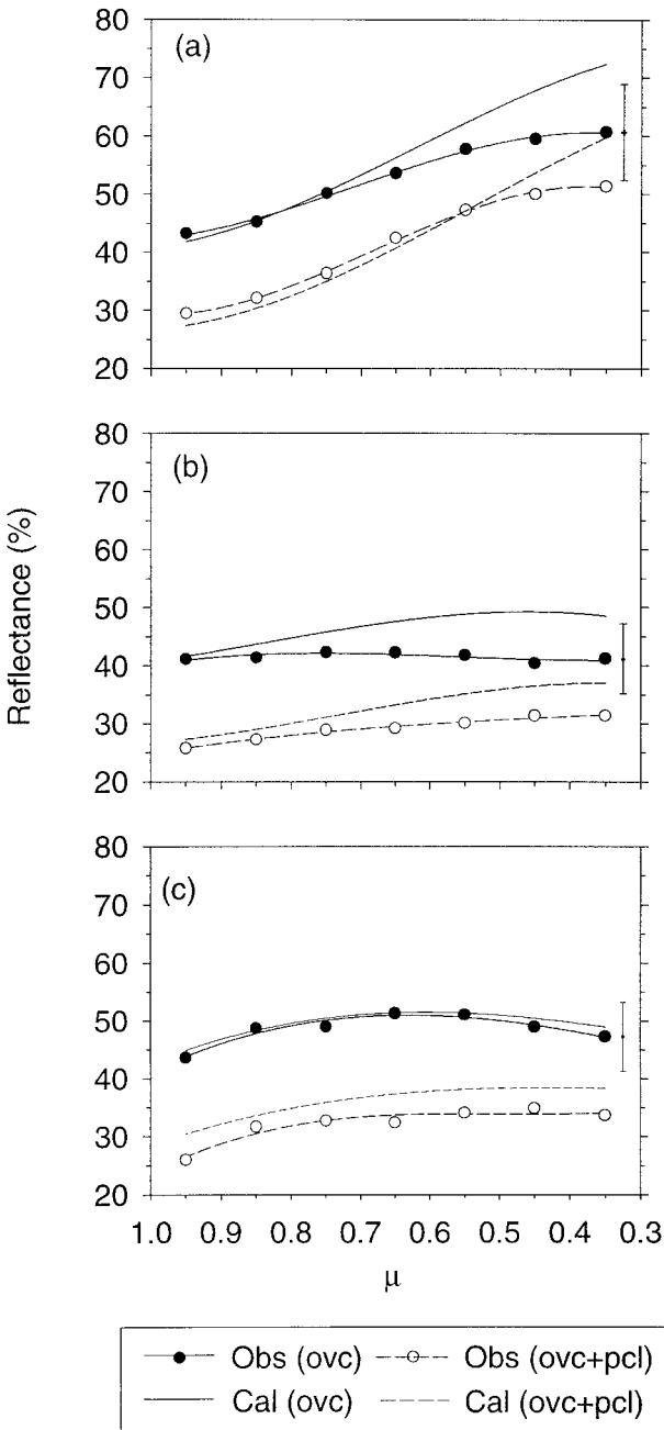
FIG. 9. Observed and calculated mean reflectances and \mu for \mu_o = 0.6-0.7 at relative azimuth (a) \phi = 10^\circ-30^\circ ; (b) \phi = 60^\circ-80^\circ ; and (c) \phi = 120^\circ-140^\circ , for NOAA-11 and NOAA-14. Results are shown for overcast pixels (ovc) and for cloud-contaminated pixels (ovc + pcl).
