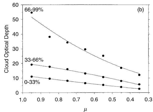
FIG. 16. Average cloud optical depths corresponding to optically thin, moderate, and thick clouds and \mu for (a) \mu_o = 0.9-1.0 and (b) \mu_o = 0.2-0.3 in the forward-scattering direction. NOAA-11 and -14 overcast observations are shown.
