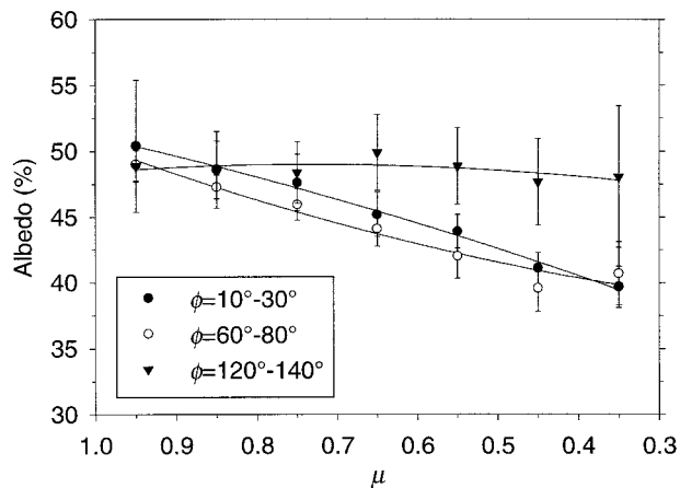
FIG. 18. Mean TOA albedo (%) and \mu at \phi = 10^\circ-30^\circ , \phi = 60^\circ-80^\circ and \phi = 120^\circ-140^\circ for the NOAA-11 and -14 ovc cases.
