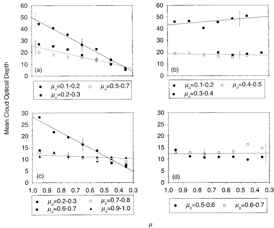
FIG. 13. Mean cloud optical depths and \mu for a range of \mu_o for overcast pixels. (a) NOAA-12 in the forward-scattering direction; (b) NOAA-12 in the backward-scattering direction; (c) NOAA-11 and -14 in the forward-scattering direction; and (d) NOAA-11 and -14 in the backward-scattering direction.
