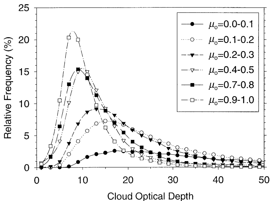
FIG. 8. Cloud optical depth distributions associated with the nadir means in Fig. 7 for the ovc case.
