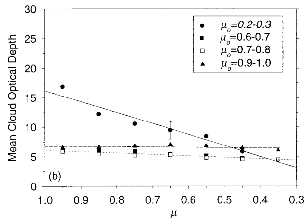
FIG. 17. Average cloud optical depths and \mu for the forward-scattering direction and various \mu_o bins for cloud-contaminated pixels. (a) NOAA-12 and (b) NOAA-11 and -14 .
