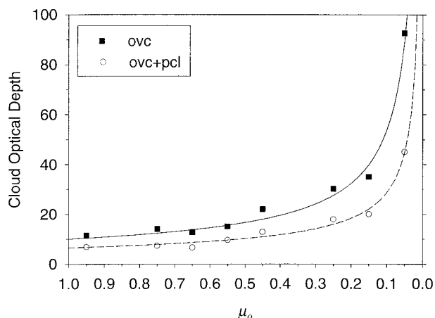
FIG. 7. Mean nadir cloud optical depths and \mu_o from NOAA-11 and -14 for overcast pixels (“ovc”) and for all cloud-contaminated pixels (“ovc + pcl”).
