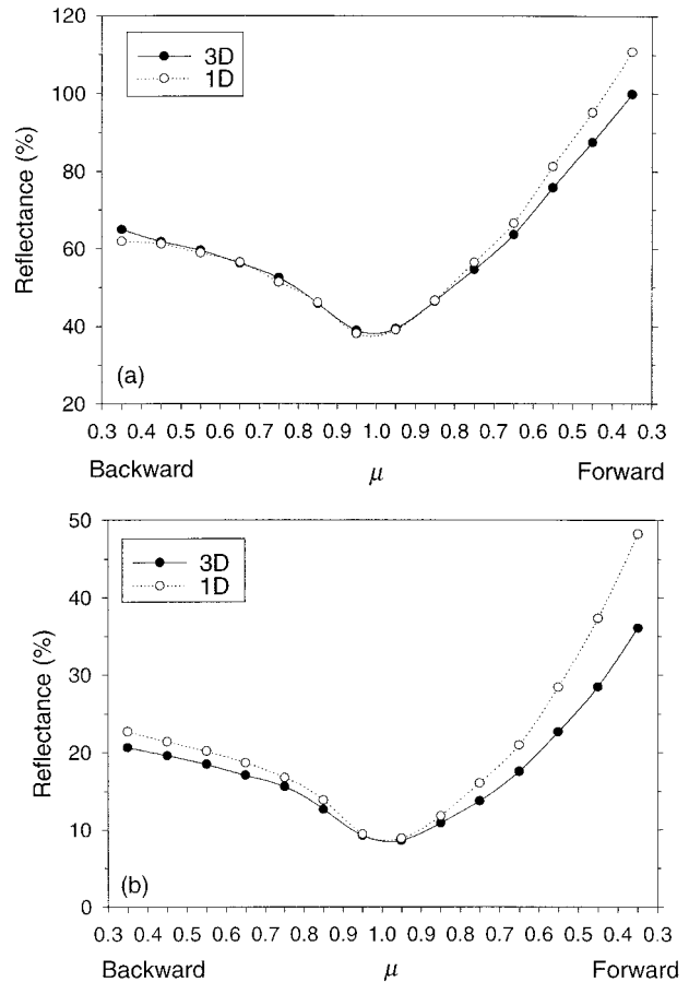
FIG. 19. Monte Carlo model simulations of 3D and 1D reflectances and \mu for overcast cloud fields with single scattering albedos ( \omega_s ) of (a) 1.0 and (b) 0.9.
