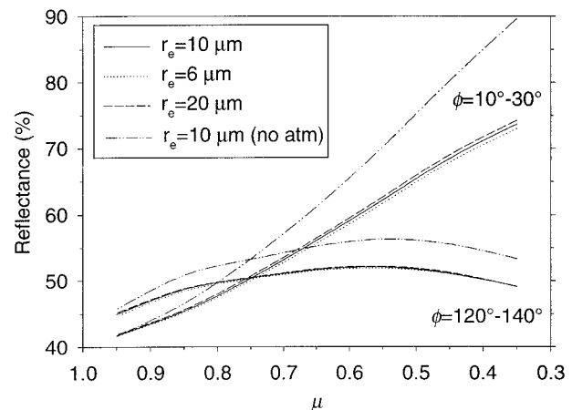
FIG. 11. Reflectances calculated for a wide range of 1D model input assumptions derived using optical depths from overcast nadir observations in the same manner as the Cal (ovc) curves in Fig. 9.
