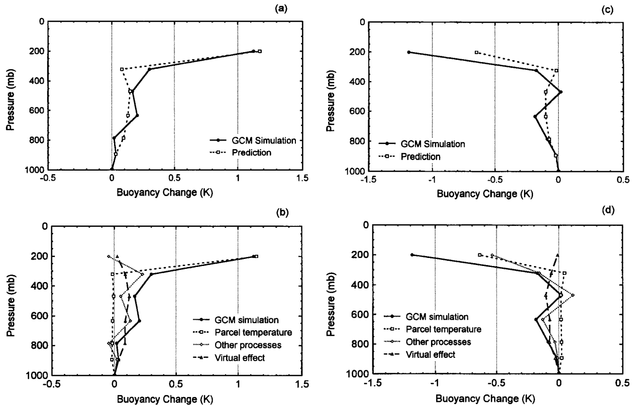
FIG. 7. (a) Changes in the vertical profiles of July monthly mean buoyancy during convection in the tropical Pacific (110°E–75°W, 26°S–26°N) for the SST +2 climate. The GISS GCM simulation is denoted by the solid line; the dashed line is for the prediction. (b) The vertical profile of July monthly mean buoyancy change as shown in (a) simulated by the GISS GCM in the SST +2 climate (solid line) is partitioned into different parts due to parcel temperature change (short dashed line with square), change in virtual effect (long dashed line with triangle), and changes in other processes (dotted line with diamond). (c) As in (a) but for the SST –2 climate. (d) As in (b) but for the SST –2 climate.
