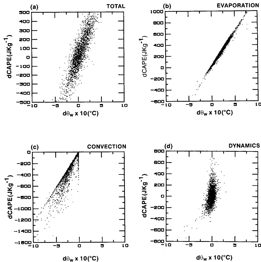
FIG. 3. Change of CAPE ( \text{J kg}^{-1} ) vs change of \Theta_w ( 10^{-1} \text{ }^\circ\text{C} ) for each GCM time step (a) due to all the physics, (b) due to surface evaporation only, (c) due to moist convection only, and (d) due to large-scale dynamics only.
