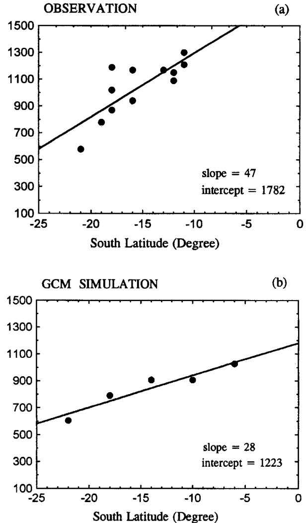
FIG. 4. (a) The dCAPE/d\Theta_w as a function of latitude observed in AMEX, adapted from Williams (1994). (b) The dCAPE/d\Theta_w as a function of latitude simulated by the GISS GCM with the prescribed SST in January 1985.
