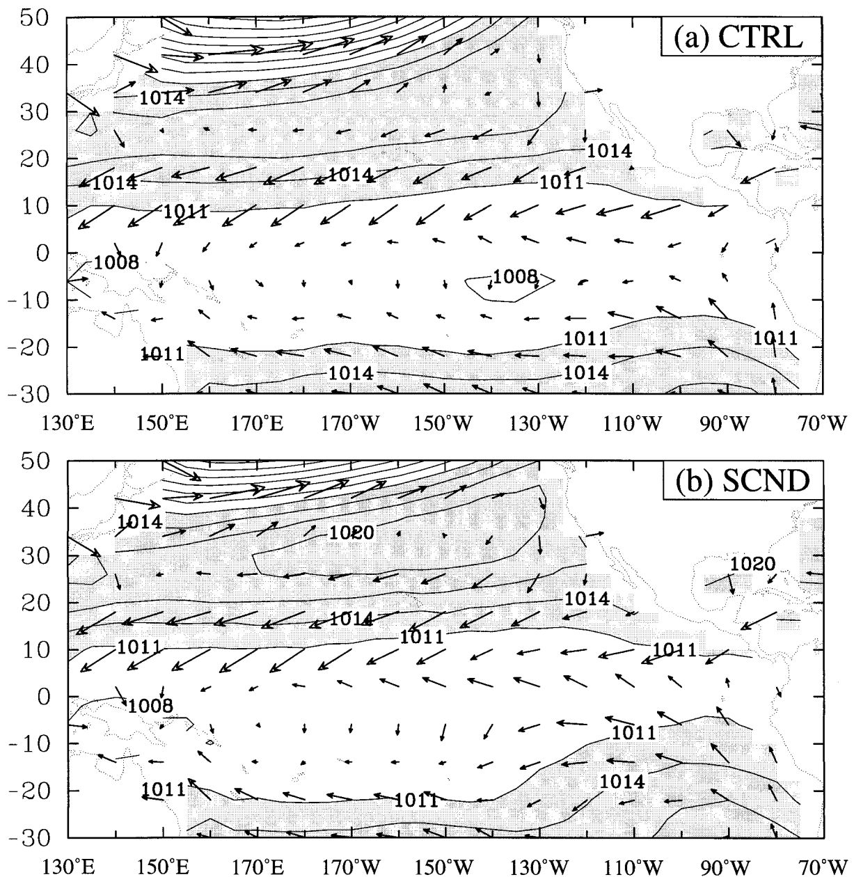
FIG. 10. Nov–Feb mean sea level pressure (contours) and PBL wind speed (arrows) from (a) the control simulation and (b) the second-half-year experiment. Contour intervals are 3 mb. Values larger than 1011 mb are shaded.
