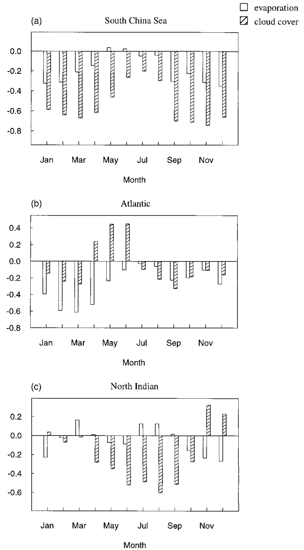
FIG. 5. Correlation coefficients for each calendar month between anomalies in evaporation (clear columns) and cloud cover (hatched columns) from ship observations (1952–92) and the ENSO index for the South China Sea, tropical north Atlantic, and Indian Ocean. The ocean areas encompassing each region are the same as in the caption to Fig. 1. Before calculation of the coefficients, the time series of evaporation and cloud cover anomalies were smoothed by a 3-month running mean and the linear trend over the 41 yr was removed.
