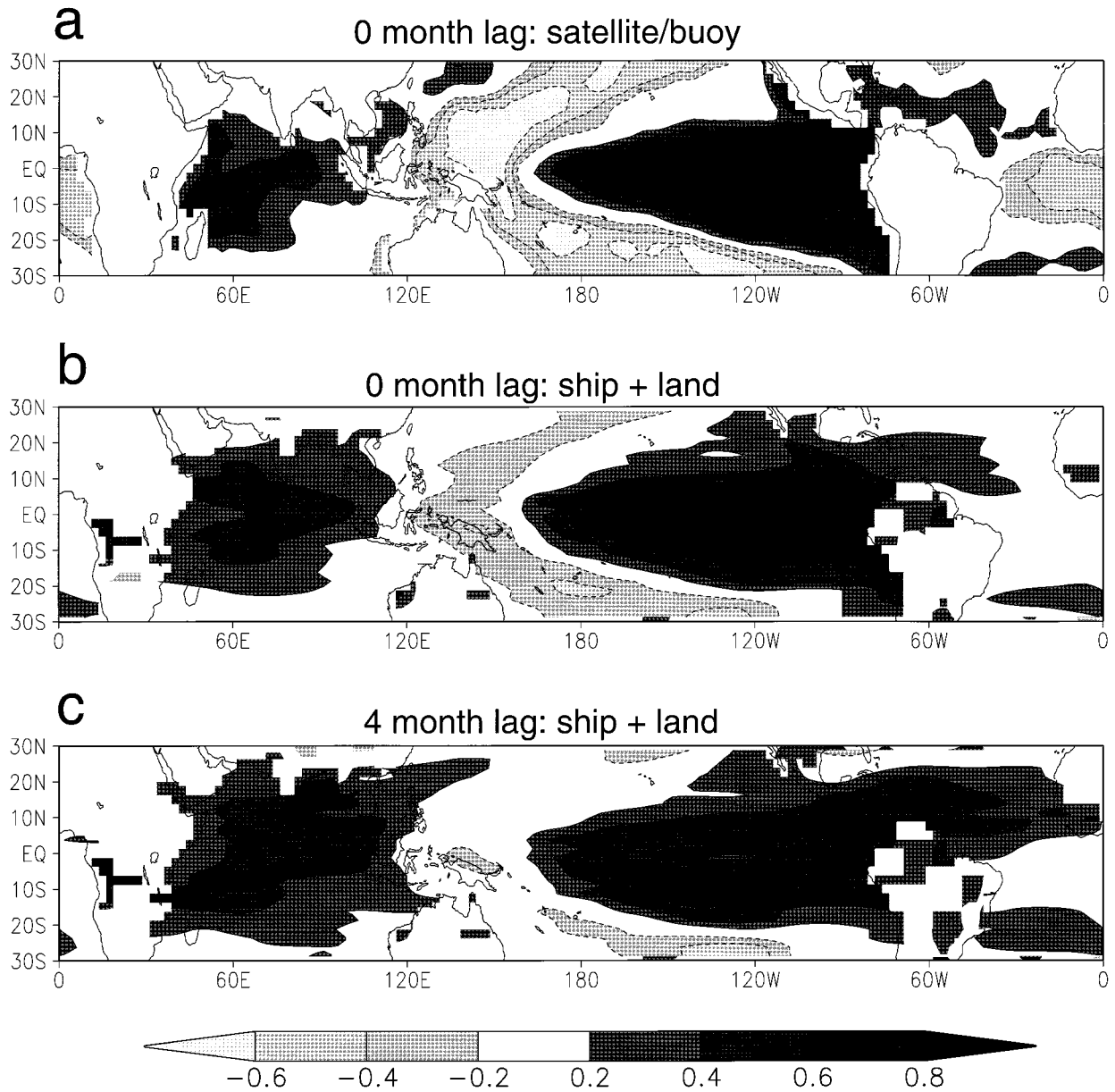
FIG. 2. Maps of correlation coefficients between SST anomalies at each point and the ENSO index. (a) The correlation coefficients between satellite SST (Reynolds 1988) and the ENSO index for the period 1982–92. (b) The correlation coefficients between ship-observed SST and the ENSO index for the period 1952–92. Also included in this panel are the correlation coefficients between surface air temperature at land stations and the ENSO index for the period 1952–90. (c) The same as (b) but with SST and surface air temperatures lagging the ENSO index by 4 months. Prior to the calculation of correlation coefficients, the data at each grid point have been smoothed using a 3-month running mean.
