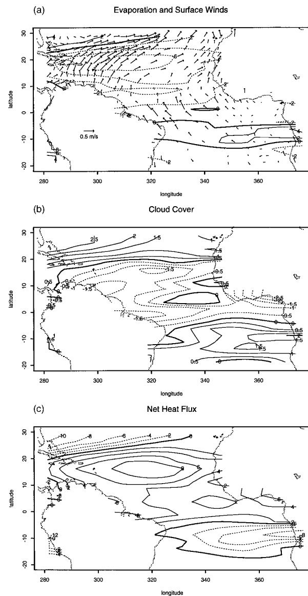
FIG. 8. As in Fig. 7 but for anomalies in the tropical Atlantic for the calendar months of January, February, March, and April in the years 1952–92. A reference wind vector is plotted over South America.
