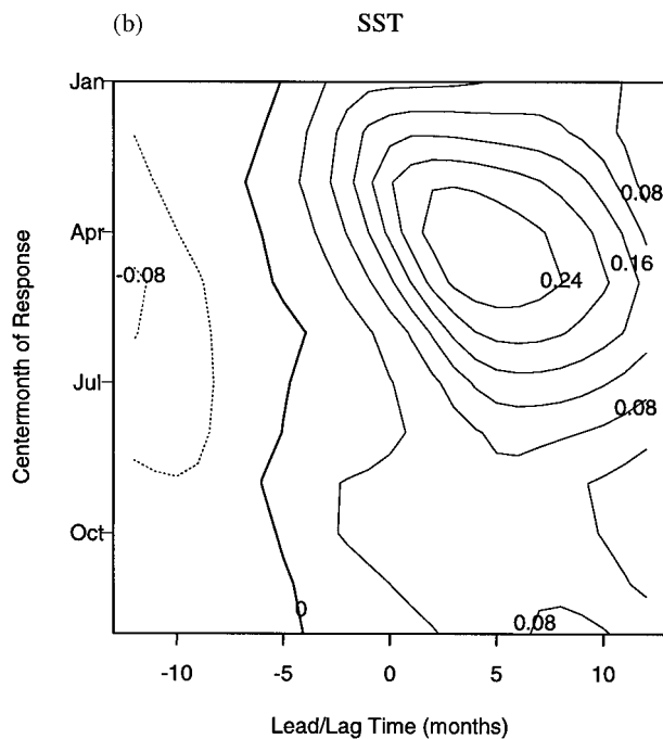
FIG. 11. As in Fig. 10 except that the time series are taken from ship observations of the inferred heat flux and SST anomalies from a portion of the tropical North Atlantic ( 5^{\circ} – 22.5^{\circ}\text{N} , 17.5^{\circ} – 60^{\circ}\text{W} ).
