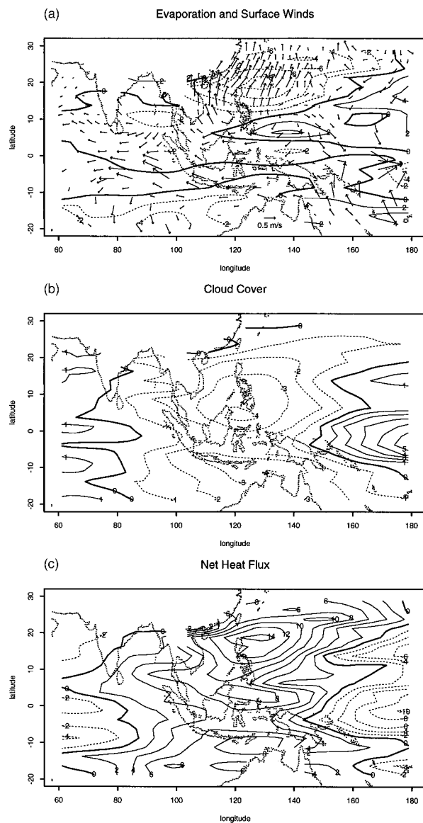
FIG. 7. Typical October–March anomalies that accompany above normal conditions of the ENSO index. (a) The anomalies in vector mean surface wind (see reference vector plotted over northern Australia) and latent heat flux, in W m^{-2} , deduced by the bulk formulas. (b) The anomalies in ship-observed cloud cover in percent. (c) The anomalies in inferred net heat flux into the ocean in W m^{-2} . The anomalies are computed by regressing the ship observations for the months of October–March in the period 1952–92 upon the ENSO index and scaling the resulting slopes by the standard deviation of the ENSO index to yield quantities with physical units. Before calculation of the anomalies, the time series of surface winds, latent heat flux, and cloud cover anomalies at each point were smoothed by use of a 3-month running mean and the linear trend over the 41 yr was removed.
