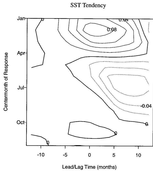
FIG. 12. As in Fig. 11 except that the time series is the SST tendency ( ^{\circ}\text{C month}^{-1} ) from a portion of the tropical North Atlantic ( 5^{\circ} – 22.5^{\circ}\text{N} , 17.5^{\circ} – 60^{\circ}\text{W} ).
