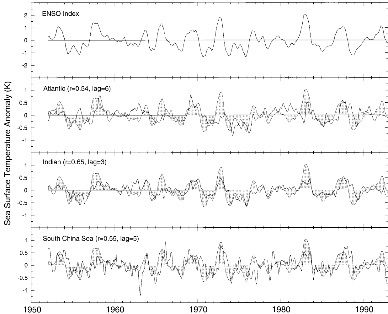
FIG. 1. Time series of the ENSO index and SST anomalies in the tropical North Atlantic ( 5^{\circ} – 22.5^{\circ} N, 17.5^{\circ} – 85^{\circ} W), Indian Ocean ( 10^{\circ} S– 25^{\circ} N, 45^{\circ} – 100^{\circ} E), and South China Sea ( 2.5^{\circ} – 22.5^{\circ} N, 100^{\circ} – 120^{\circ} E). For each time series, the data have been smoothed using a 3-month running mean and the linear trend over the 41 yr has been removed. The shaded curve plotted with each SST time series is the ENSO index divided by 2. Above each SST time series is the value of the correlation coefficient between the ENSO index and the SST time series at the lag time corresponding to the maximum correlation coefficient. For example, the North Atlantic Ocean time series has a correlation coefficient of +0.54 with the ENSO index when the North Atlantic Ocean time series lags the ENSO index by 6 months.
