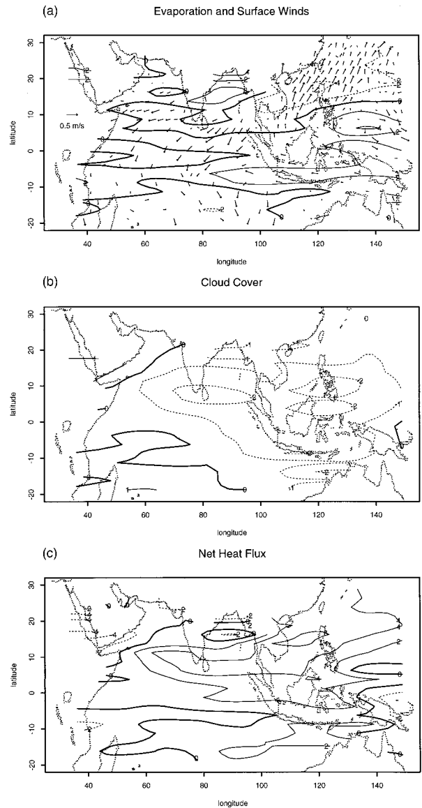
FIG. 9. As in Fig. 7 but for anomalies in the Indian Ocean for the calendar months of April, May, June, July, August, and September in the years 1952–92. The regression was performed with the ENSO index lagging the anomalies by 3 months. A reference wind vector is plotted over eastern Africa.
