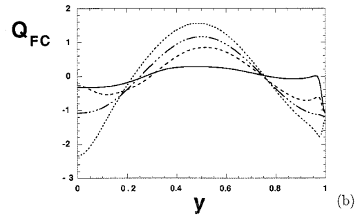
FIG. 6. (a) Contour plot of the flux-correction freshwater flux forcing Q_{FC}(y) as a function of latitude (scaled by domain length) and Ra. This is the flux required to maintain the true surface salinity field S_T , even when model parameters (here only Ra) differ from the true values. The field is scaled by its absolute maximum and contour levels are with respect to this maximum. (b) Sections at different values of Ra, with Ra = 7.56 \times 10^2 (solid), Ra = 5.35 \times 10^3 (dashed), Ra = 9.54 \times 10^3 (dash-dotted), and Ra = 1.77 \times 10^4 (dotted).
