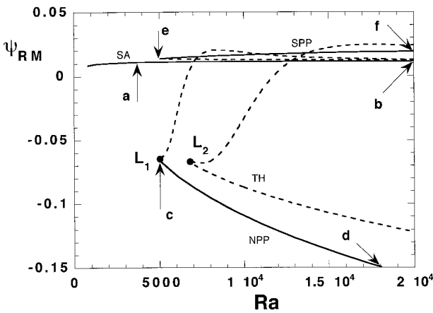
FIG. 3. Bifurcation diagram in Ra for \sigma = 0.128 with the forcing Q_T and T_0 and standard values of other parameters. Format as in Fig. 1. Labels a–f indicate points for which solutions are shown in Fig. 4.
