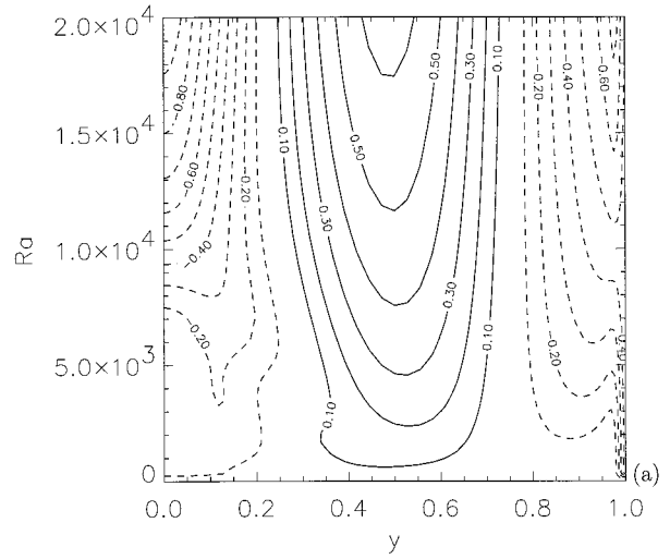
FIG. 5. Bifurcation diagram in Ra for restoring boundary conditions that fix surface salinity and temperature to S_T and T_0 and standard values of parameters with \sigma = 0.128 . Format as in Fig. 1.
