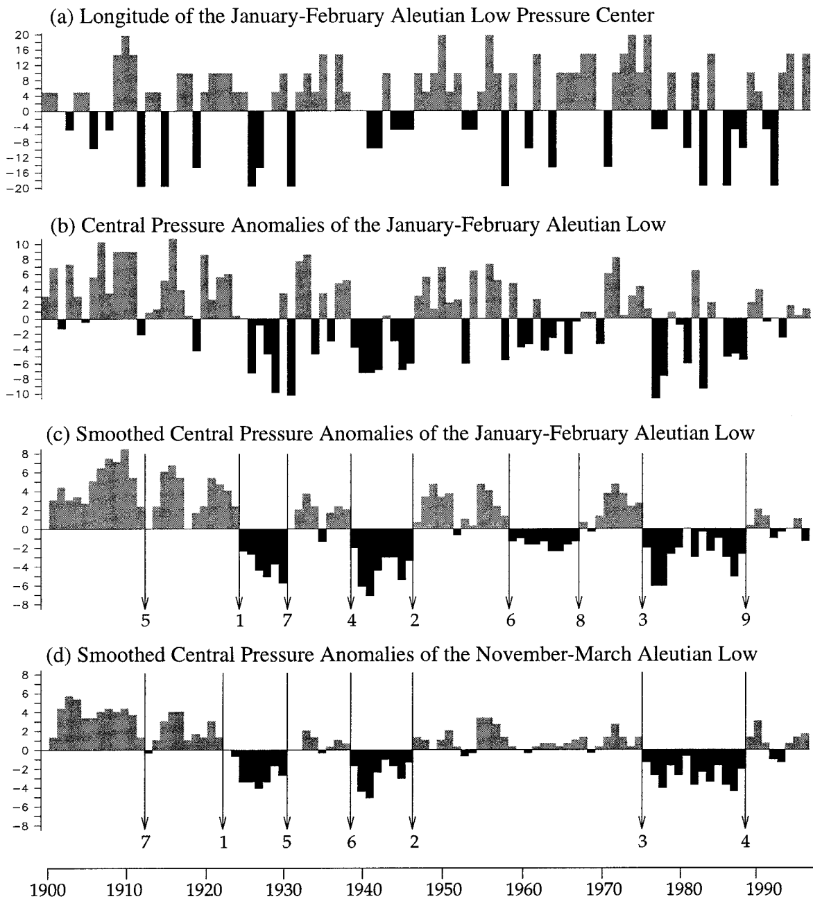
FIG. 1. Characteristics of the Aleutian low for 1900–96. (a) Long of the Jan–Feb Aleutian low pressure center, plotted as degrees west (positive) or east (negative) of 180°; (b) central pressure anomalies of the Jan–Feb Aleutian low, in mb; (c) as in (b) but smoothed with a 3-yr running mean; (d) central pressure anomalies of the Nov–Mar Aleutian low, smoothed with a 3-yr running mean. Numbered arrows in (c) and (d) indicate the objectively determined change points and the order in which they were detected. See text for a discussion on the significance of the change points. Data are from the NHSLP dataset; pressure anomalies are based on a 1946–96 climatology.
