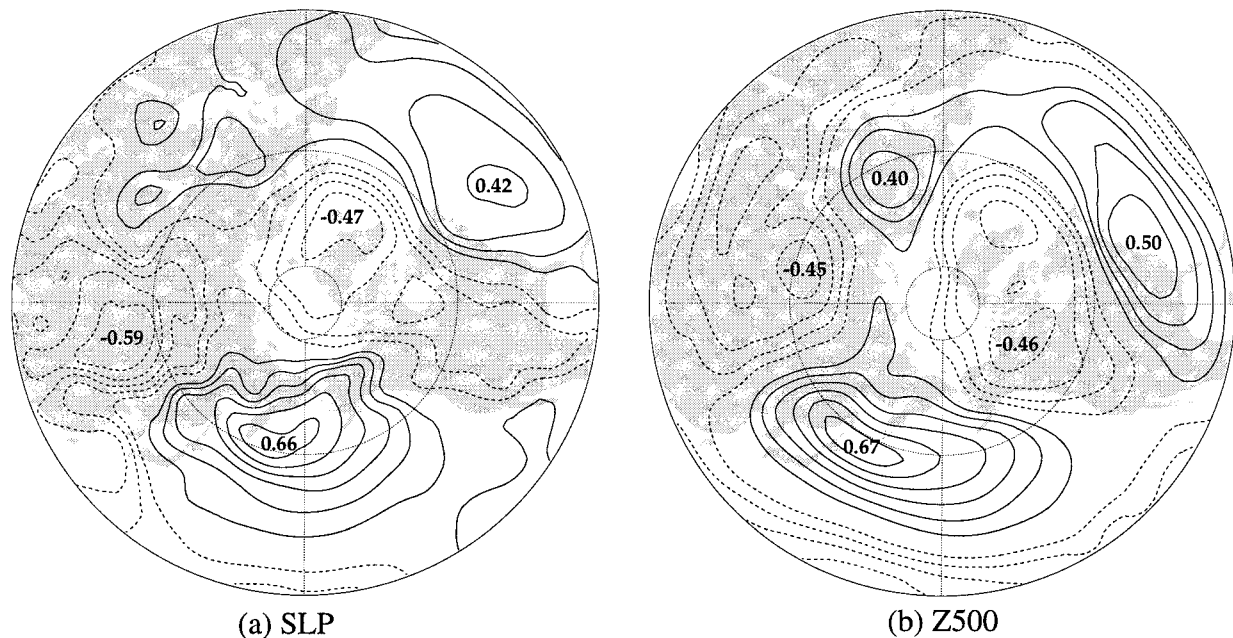
FIG. 2. Correlation maps for the Jan–Feb Aleutian low central pressure index (plotted in Fig. 1c) and (a) Jan–Feb mean sea level pressure, and (b) Jan–Feb mean 500-mb height. The contour interval is 0.1, with negative correlations plotted with dashed lines and positive correlations plotted with solid lines. Printed numbers indicate local maxima and minima. Latitude circles are drawn at 20°, 50°, and 80°N.
