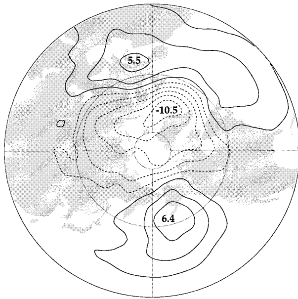
FIG. 4. Hemispheric map showing the changes in the Jan–Feb mean SLP, 1989–97 minus 1977–88. The contour interval is 2 mb, centered on zero, with negative values plotted with dashed lines and positive values plotted with solid lines. Printed numbers indicate local maxima and minima. Monthly mean data are from the NCEP–NCAR reanalysis dataset.
