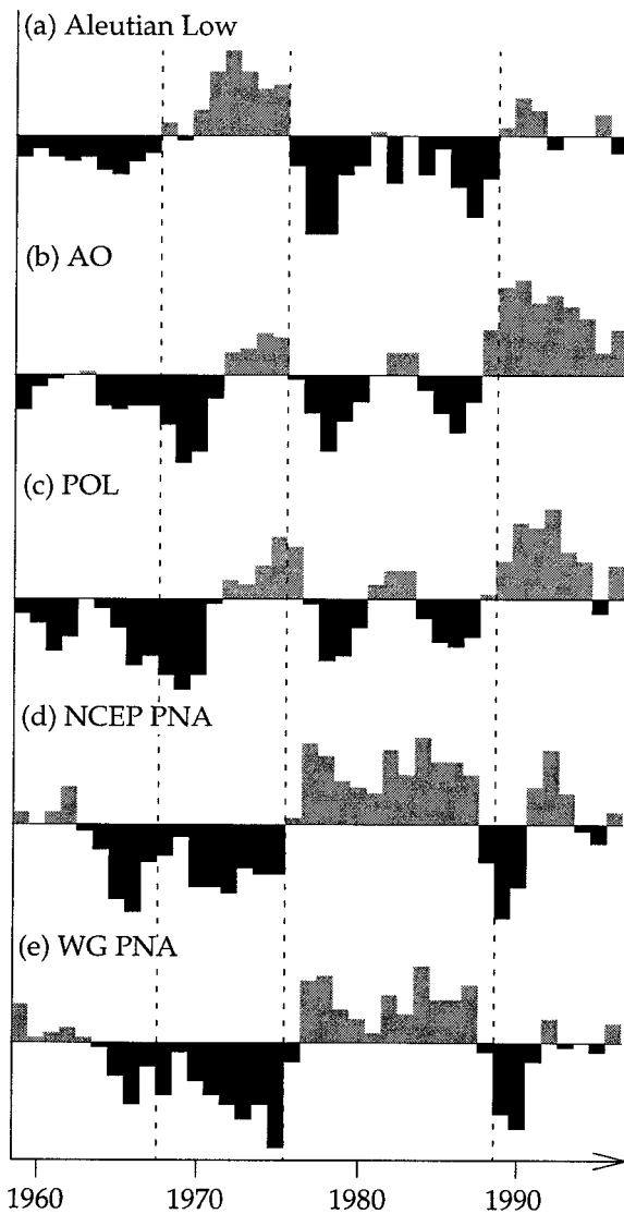
FIG. 3. (a) Central pressure anomalies of the Jan–Feb Aleutian low; (b)–(e) Jan–Feb averages of the amplitudes of the following indices: Arctic Oscillation (AO), the NCEP Polar–Eurasia (POL), the NCEP Pacific–North America (PNA), and the Wallace–Gutzler (WG) PNA. All time series span the period from 1959 to 1996 and have been smoothed with a 3-yr running mean. Dashed lines indicate the zero crossings of the Aleutian low central pressure anomalies in 1967, 1976, and 1989.
