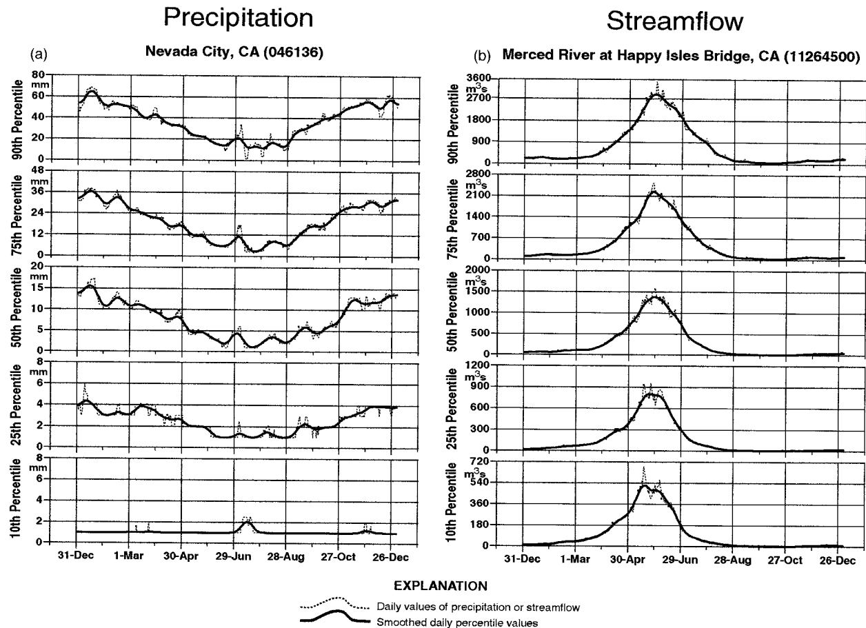
Fig. 4. Smoothed percentiles of (a) daily precipitation, Nevada City, CA, and (b) nearby daily stream flow on the Merced River at Happy Isles Bridge, CA, based on 1948–95 data.
