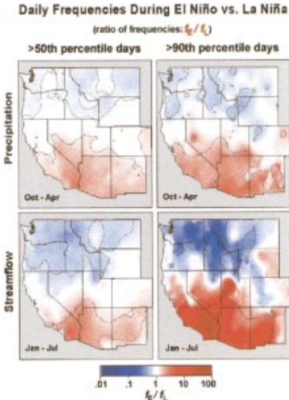
FIG. 7. (a) and (b) Precipitation and (c) and (d) stream flow f_E/f_L ratio of frequencies (SOI–/SOI+) of daily values exceeding (a) and (c) 50th percentile and (b) and (d) 90th percentile. Precipitation during Oct–Apr, stream flow during Jan–Jul, 1948–95. Red denotes ratios >1.0 (SOI– cases have more frequent events than SOI+ cases), blue denotes ratios <1.0 (SOI– cases have less frequent events than SOI+ cases). Dashed lines denote regions where frequency ratio exceeds 90% confidence levels via Monte Carlo trials.
