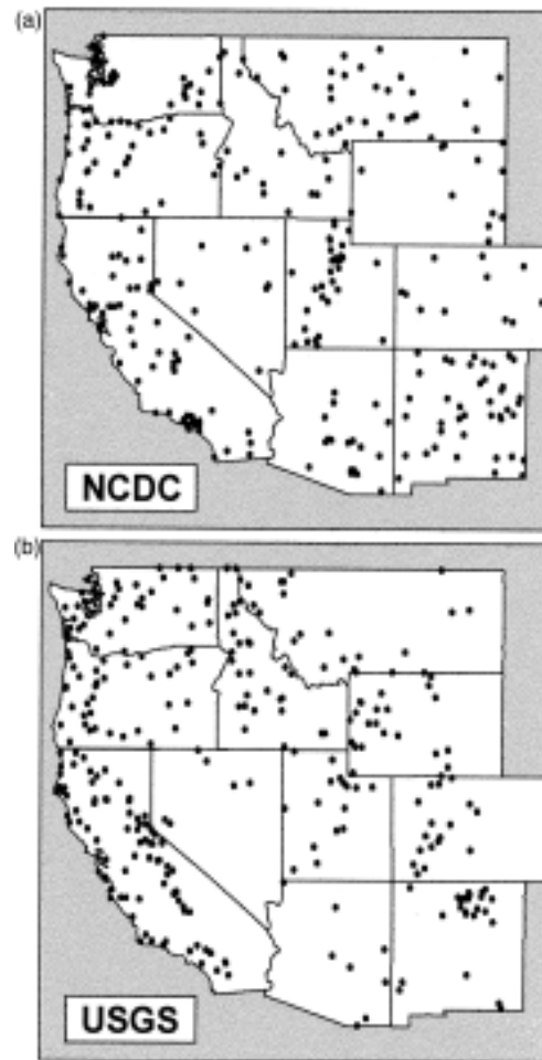
FIG. 3. Areal distribution of selected (a) NCDC precipitation stations and of (b) USGS stream gauges.
