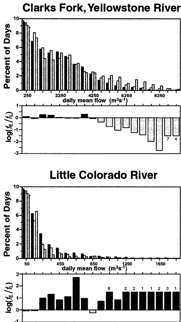
FIG. 6. Frequency distribution of daily mean stream flow for SOI - and SOI + for (a) Clark's Fork River of the Yellowstone River, near Belfry, MT, and (c) for the Little Colorado River above Lyman Lake, AZ. Based on Jan–Jul, 1948–95, the lowest category of flow in (a) and (c) is truncated in order to display higher flow categories. (b) and (c) Graph of each pair shows ratio of frequency, SOI - /SOI + ; when ratio is infinite (one category has no occurrences), the value plotted is 1.5, and the number of occurrences in the other category is labeled at top of bar.
