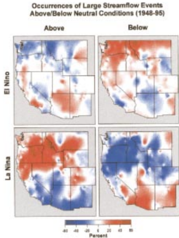
FIG. 10. Differences in fraction of years within category of daily P90 stream flow above/below expected from tercile boundaries of neutral year cases. (a) and (b) SOI - (El Niño) minus neutral and (c) and (d) SOI + (La Niña) minus neutral. Values are the difference in percent of total years having above expected or below expected number of P90 events.
