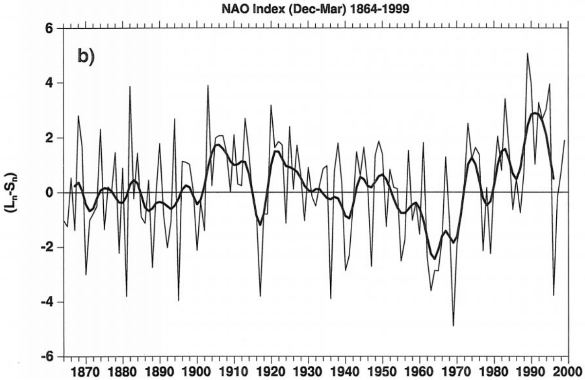
FIG. 1. (a) The first EOF of winter SLP for the North Atlantic sector based on Trenberth and Paolino (1980), and created from DJFM means over the period 1899–1977. The EOF is based on the covariance matrix and explains 34% of the variance. (b) The winter (DJFM) NAO index, updated from Hurrell (1995a).
